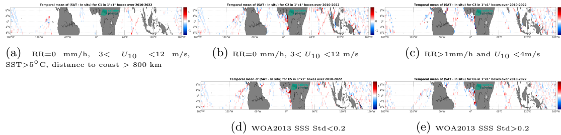
Figure 12: Temporal mean gridded over spatial boxes of size 1^\circ \times 1^\circ of \Delta SSS (SMOS SSS L3 v8 - 9 Days (CATDS-CEC-LOCEAN) - TSG (LEGOS-DM)) for 5 different subdatasets corresponding to: RR=0 mm/h, 3 < U_{10} < 12 m/s, SST >5^\circ C, distance to coast > 800 km (a), RR=0 mm/h, 3 < U_{10} < 12 m/s (b), RR >1 mm/h and U_{10} < 4 m/s (c), WOA2013 SSS Std <0.2 (d), WOA2013 SSS Std >0.2 (e).
