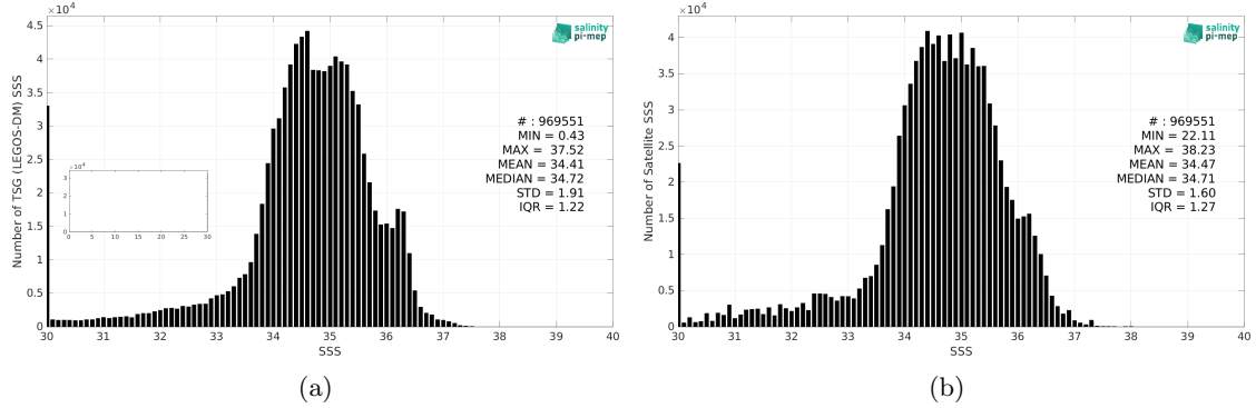
Figure 2: Histograms of SSS from TSG (LEGOS-DM) (a) and SMOS SSS L3 v8 - 9 Days (CATDS-CEC-LOCEAN) (b) considering all match-up pairs per bins of 0.1 over the Equatorial Ocean 10N-10S Pi-MEP region and for the full satellite product period.
