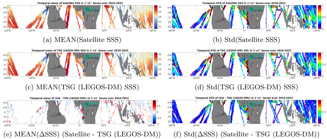
Figure 6: Temporal mean (left) and Std (right) of SSS from SMOS SSS L3 v8 - 9 Days (CATDS-CEC-LOCEAN) (top), TSG (LEGOS-DM) (middle), and of \Delta SSS (Satellite - TSG (LEGOS-DM)). Only match-up pairs are used to generate these maps.
