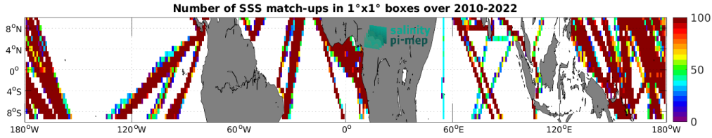
Figure 4: Number of SSS match-ups between TSG (LEGOS-DM) SSS and the SMOS SSS L3 v8 - 9 Days (CATDS-CEC-LOCEAN) SSS product for the Equatorial Ocean 10N-10S Pi-MEP region over 1^\circ \times 1^\circ boxes and for the full satellite product period.
