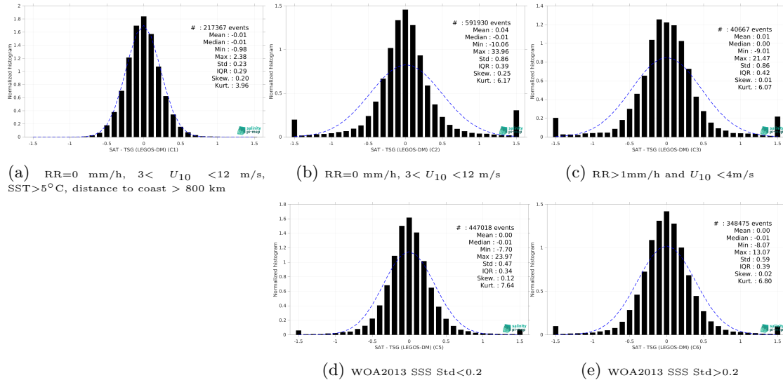
Figure 13: Normalized histogram of \Delta SSS (SMOS SSS L3 v8 - 9 Days (CATDS-CEC-LOCEAN) - TSG (LEGOS-DM)) for 5 different subdatasets corresponding to: RR=0 mm/h, 3 < U_{10} < 12 m/s, SST >5^\circ C, distance to coast > 800 km (a), RR=0 mm/h, 3 < U_{10} < 12 m/s (b), RR >1 mm/h and U_{10} < 4 m/s (c), WOA2013 SSS Std <0.2 (d), WOA2013 SSS Std >0.2 (e).
