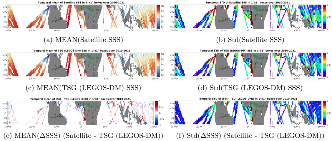
Figure 6: Temporal mean (left) and Std (right) of SSS from SMOS SSS L3 v8 - 9 Days (CATDS-CECOS-LOCEAN) (top), TSG (LEGOS-DM) (middle), and of \Delta SSS (Satellite - TSG (LEGOS-DM)). Only match-up pairs are used to generate these maps.
