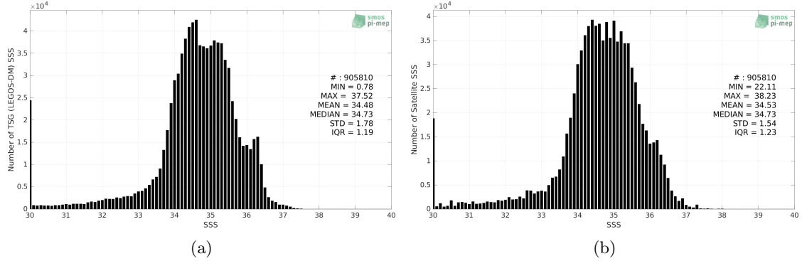
Figure 2: Histograms of SSS from TSG (LEGOS-DM) (a) and SMOS SSS L3 v8 - 9 Days (CATDS-CECOS-LOCEAN) (b) considering all match-up pairs per bins of 0.1 over the Equatorial Ocean 10N-10S Pi-MEP region and for the full satellite product period.
