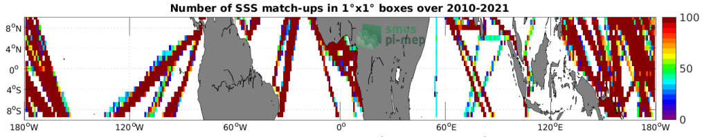
Figure 4: Number of SSS match-ups between TSG (LEGOS-DM) SSS and the SMOS SSS L3 v8 - 9 Days (CATDS-CECOS-LOCEAN) SSS product for the Equatorial Ocean 10N-10S Pi-MEP region over 1^\circ \times 1^\circ boxes and for the full satellite product period.
