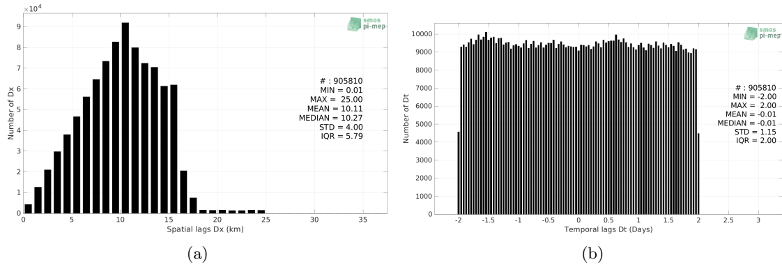
Figure 5: Histograms of the spatial (a) and temporal (b) lags between the location/time of the TSG (LEGOS-DM) measurement and the date of the corresponding SMOS SSS L3 v8 - 9 Days (CATDS-CECOS-LOCEAN) SSS pixel.
