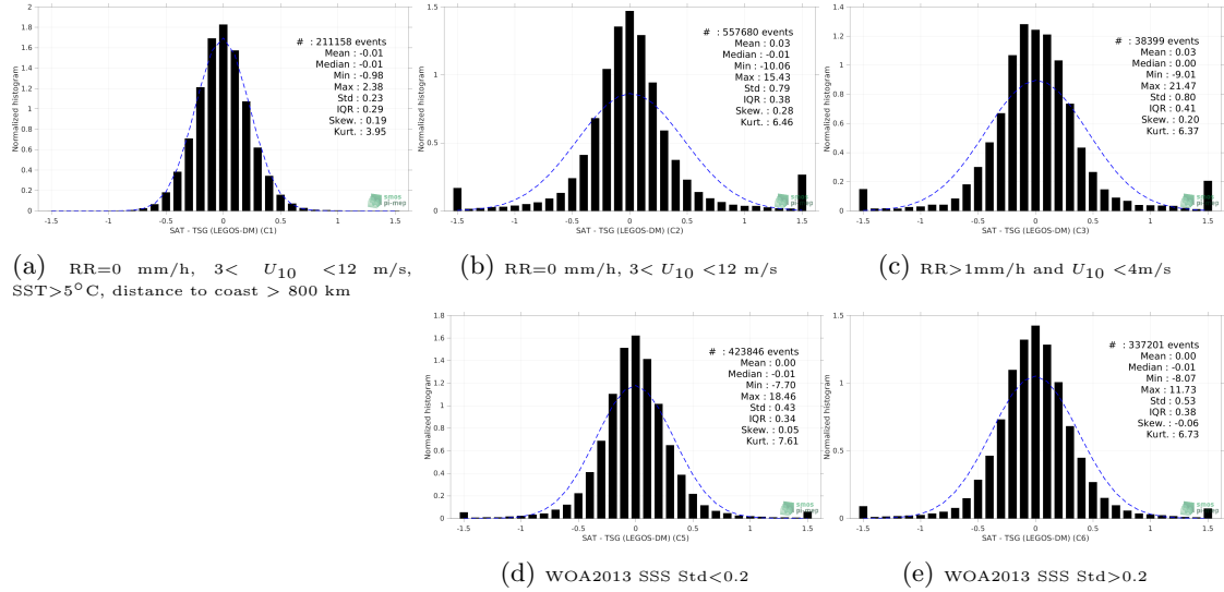
Figure 13: Normalized histogram of \Delta SSS (SMOS SSS L3 v8 - 9 Days (CATDS-CECOS-LOCEAN) - TSG (LEGOS-DM)) for 5 different subdatasets corresponding to: RR=0 mm/h, 3 < U_{10} < 12 m/s, SST>5°C, distance to coast > 800 km (a), RR=0 mm/h, 3 < U_{10} < 12 m/s (b), RR>1mm/h and U_{10} < 4 m/s (c), WOA2013 SSS Std<0.2 (d), WOA2013 SSS Std>0.2 (e).
