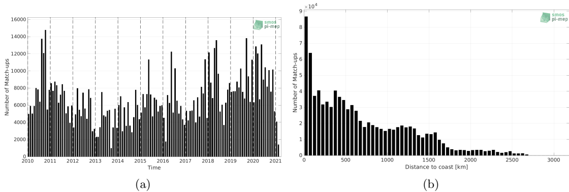
Figure 1: Number of match-ups between TSG (LEGOS-DM) and SMOS SSS L3 v8 - 9 Days (CATDS-CECOS-LOCEAN) SSS as a function of time (a) and as function of the distance to coast (b) over the Equatorial Ocean 10N-10S Pi-MEP region and for the full satellite product period.
