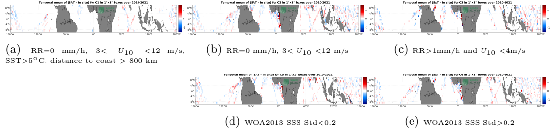
Figure 12: Temporal mean gridded over spatial boxes of size 1^{\circ}\times 1^{\circ} of \Delta\text{SSS} (SMOS SSS L3 v8 - 9 Days (CATDS-CECOS-LOCEAN) - TSG (LEGOS-DM)) for 5 different subdatasets corresponding to:RR=0 mm/h, 3 < U_{10} < 12 m/s, SST >5^{\circ}\text{C} , distance to coast > 800 km (a), RR=0 mm/h, 3 < U_{10} < 12 m/s (b), RR >1 mm/h and U_{10} < 4 m/s (c), WOA2013 SSS Std <0.2 (d), WOA2013 SSS Std >0.2 (e).
