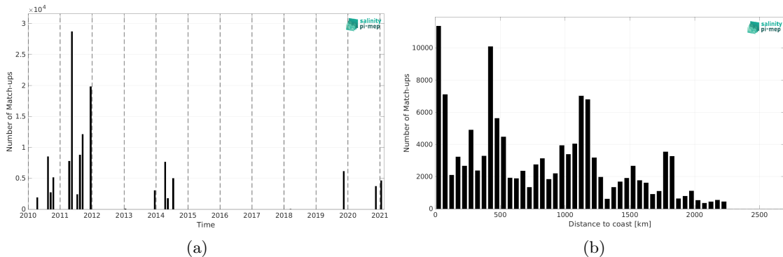
Figure 1: Number of match-ups between TSG (GOSUD-Sailing-ship) and SMOS SSS L3 v8 - 9 Days (CATDS-CEC-LOCEAN) SSS as a function of time (a) and as function of the distance to coast (b) over the Equatorial Ocean 10N-10S Pi-MEP region and for the full satellite product period.
