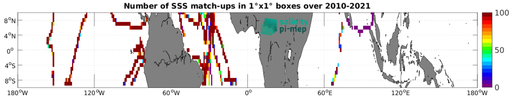
Figure 4: Number of SSS match-ups between TSG (GOSUD-Sailing-ship) SSS and the SMOS SSS L3 v8 - 9 Days (CATDS-CEC-LOCEAN) SSS product for the Equatorial Ocean 10N-10S Pi-MEP region over 1^\circ \times 1^\circ boxes and for the full satellite product period.
