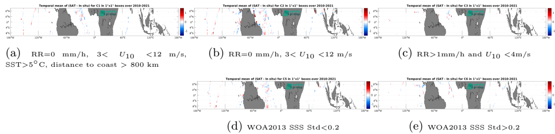
Figure 12: Temporal mean gridded over spatial boxes of size 1^{\circ}\times 1^{\circ} of \Delta SSS (SMOS SSS L3 v8 - 9 Days (CATDS-CEC-LOCEAN) - TSG (GOSUD-Sailing-ship)) for 5 different subdatasets corresponding to:RR=0 mm/h, 3 < U_{10} < 12 m/s, SST >5^{\circ}\text{C} , distance to coast > 800 km (a), RR=0 mm/h, 3 < U_{10} < 12 m/s (b), RR >1 mm/h and U_{10} < 4 m/s (c), WOA2013 SSS Std <0.2 (d), WOA2013 SSS Std >0.2 (e).
