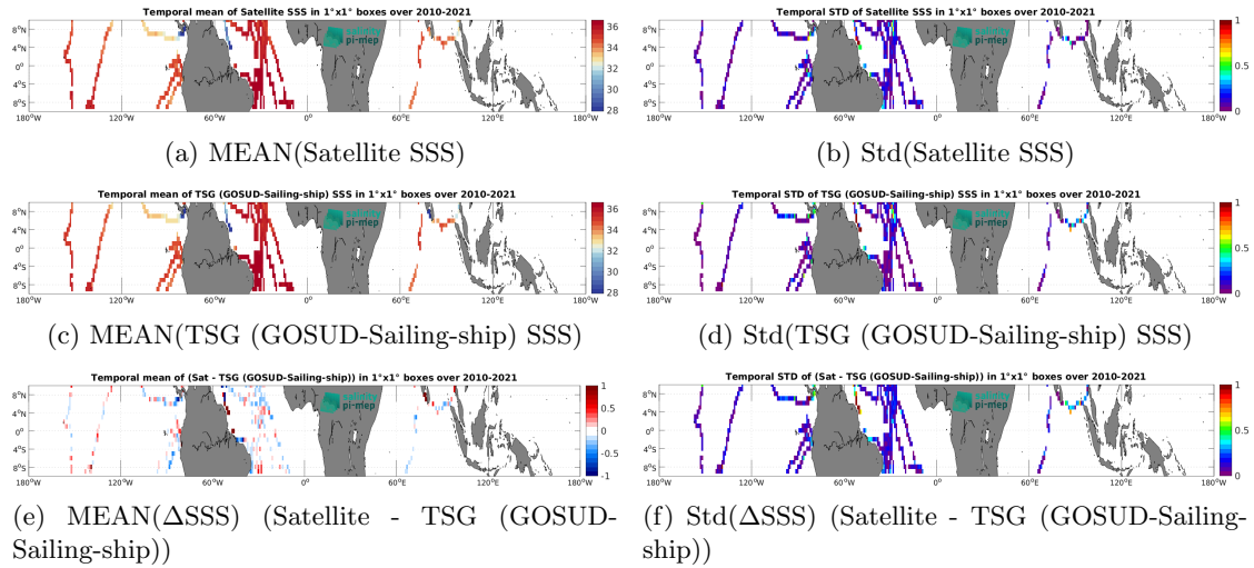
Figure 6: Temporal mean (left) and Std (right) of SSS from SMOS SSS L3 v8 - 9 Days (CATDS-CEC-LOCEAN) (top), TSG (GOSUD-Sailing-ship) (middle), and of \Delta SSS (Satellite - TSG (GOSUD-Sailing-ship)). Only match-up pairs are used to generate these maps.
