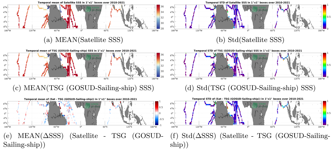
Figure 6: Temporal mean (left) and Std (right) of SSS from SMOS SSS L3 v8 - 9 Days (CATDS-CECOS-LOCEAN) (top), TSG (GOSUD-Sailing-ship) (middle), and of \Delta SSS (Satellite - TSG (GOSUD-Sailing-ship)). Only match-up pairs are used to generate these maps.
