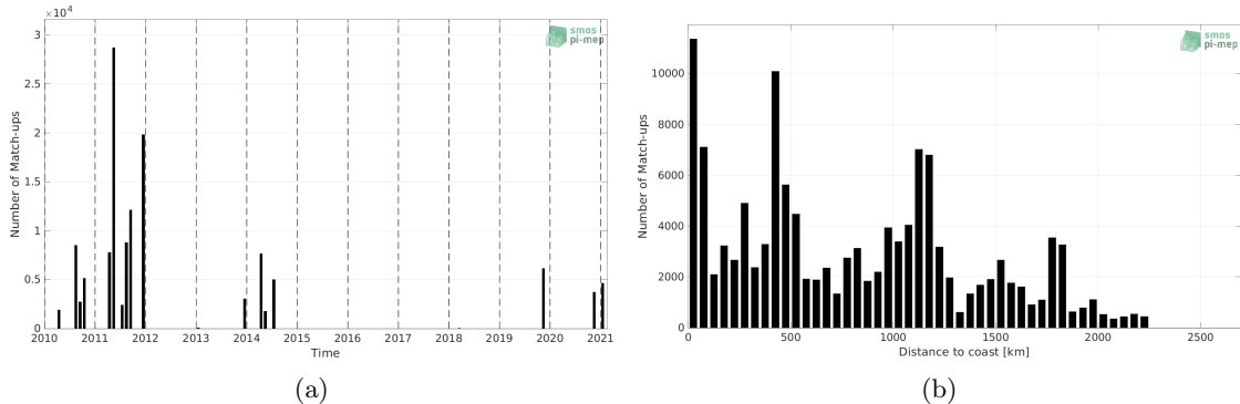
Figure 1: Number of match-ups between TSG (GOSUD-Sailing-ship) and SMOS SSS L3 v8 - 9 Days (CATDS-CECOS-LOCEAN) SSS as a function of time (a) and as function of the distance to coast (b) over the Equatorial Ocean 10N-10S Pi-MEP region and for the full satellite product period.
