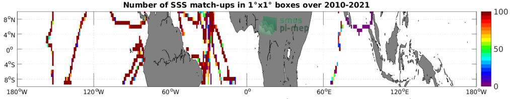
Figure 4: Number of SSS match-ups between TSG (GOSUD-Sailing-ship) SSS and the SMOS SSS L3 v8 - 9 Days (CATDS-CECOS-LOCEAN) SSS product for the Equatorial Ocean 10N-10S Pi-MEP region over 1^\circ \times 1^\circ boxes and for the full satellite product period.
