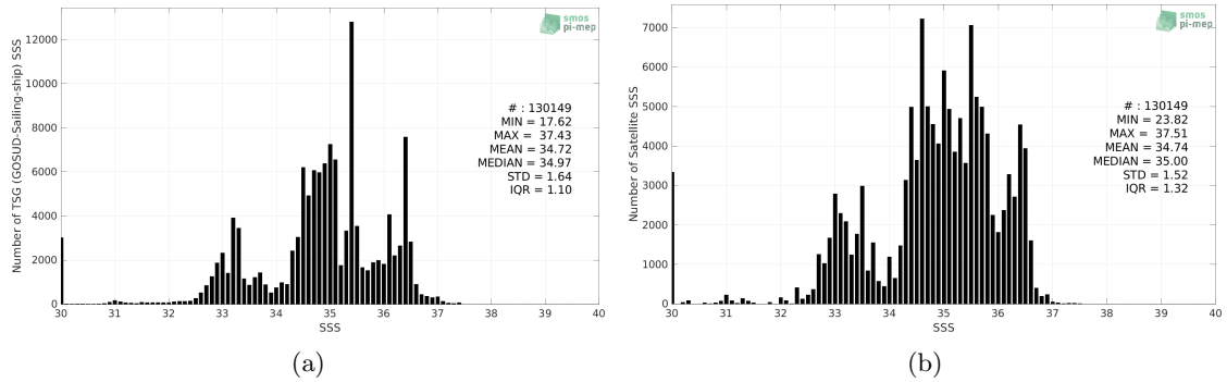
Figure 2: Histograms of SSS from TSG (GOSUD-Sailing-ship) (a) and SMOS SSS L3 v8 - 9 Days (CATDS-CECOS-LOCEAN) (b) considering all match-up pairs per bins of 0.1 over the Equatorial Ocean 10N-10S Pi-MEP region and for the full satellite product period.
