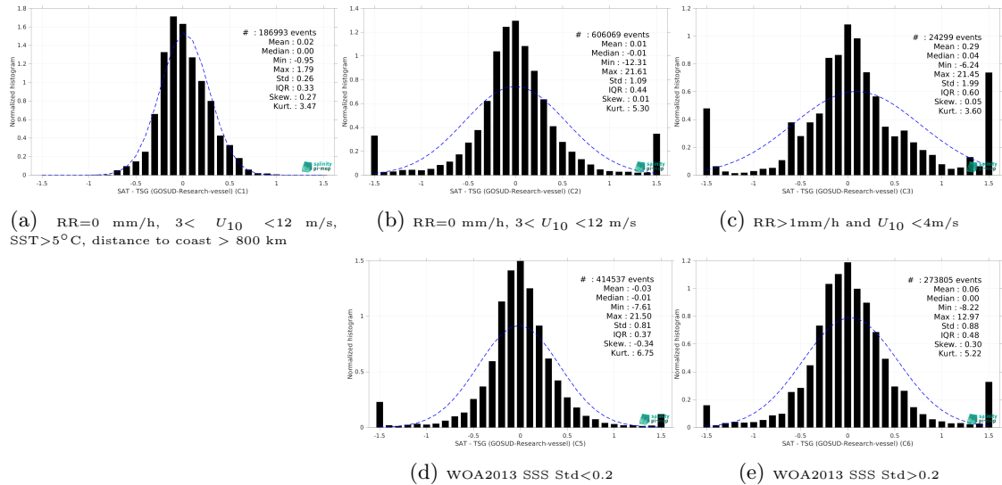
Figure 13: Normalized histogram of \Delta\text{SSS} (SMOS SSS L3 v8 - 9 Days (CATDS-CEC-LOCEAN) - TSG (GOSUD-Research-vessel)) for 5 different subdatasets corresponding to: RR=0 mm/h, 3 < U_{10} < 12 m/s, SST>5°C, distance to coast > 800 km (a), RR=0 mm/h, 3 < U_{10} < 12 m/s (b), RR>1mm/h and U_{10} < 4 m/s (c), WOA2013 SSS Std<0.2 (d), WOA2013 SSS Std>0.2 (e).
