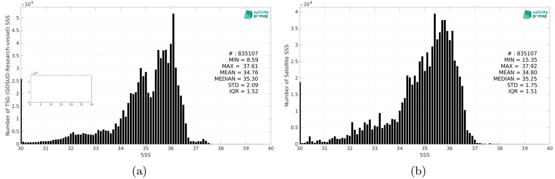
Figure 2: Histograms of SSS from TSG (GOSUD-Research-vessel) (a) and SMOS SSS L3 v8 - 9 Days (CATDS-CEC-LOCEAN) (b) considering all match-up pairs per bins of 0.1 over the Equatorial Ocean 10N-10S Pi-MEP region and for the full satellite product period.
