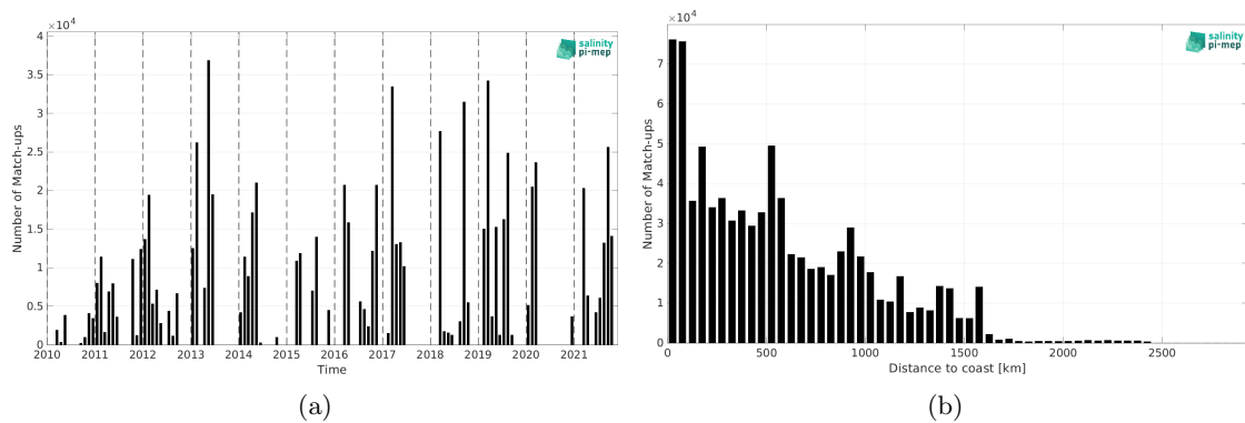
Figure 1: Number of match-ups between TSG (GOSUD-Research-vessel) and SMOS SSS L3 v8 - 9 Days (CATDS-CEC-LOCEAN) SSS as a function of time (a) and as function of the distance to coast (b) over the Equatorial Ocean 10N-10S Pi-MEP region and for the full satellite product period.
