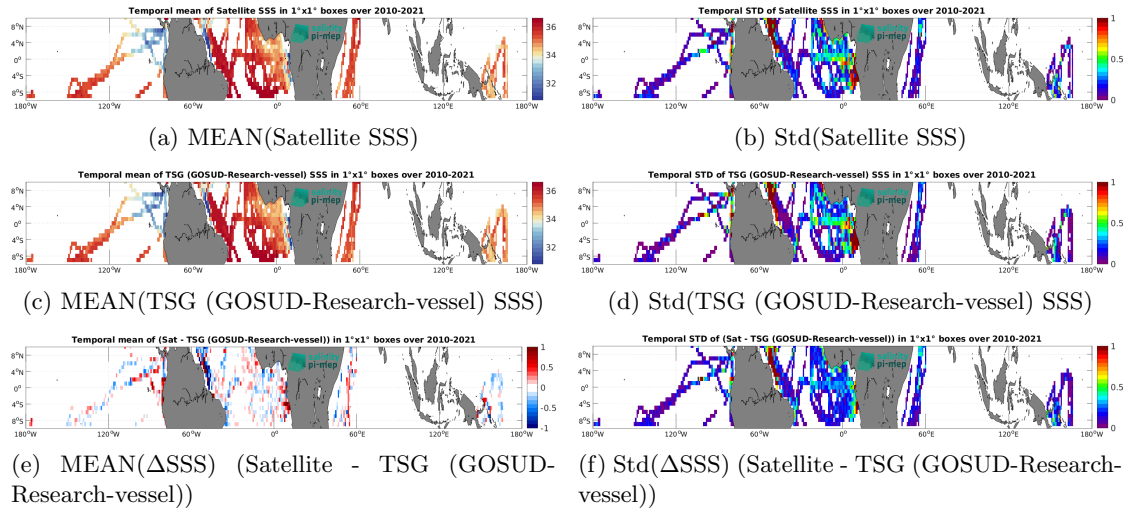
Figure 6: Temporal mean (left) and Std (right) of SSS from SMOS SSS L3 v8 - 9 Days (CATDS-CEC-LOCEAN) (top), TSG (GOSUD-Research-vessel) (middle), and of \Delta SSS (Satellite - TSG (GOSUD-Research-vessel)). Only match-up pairs are used to generate these maps.
