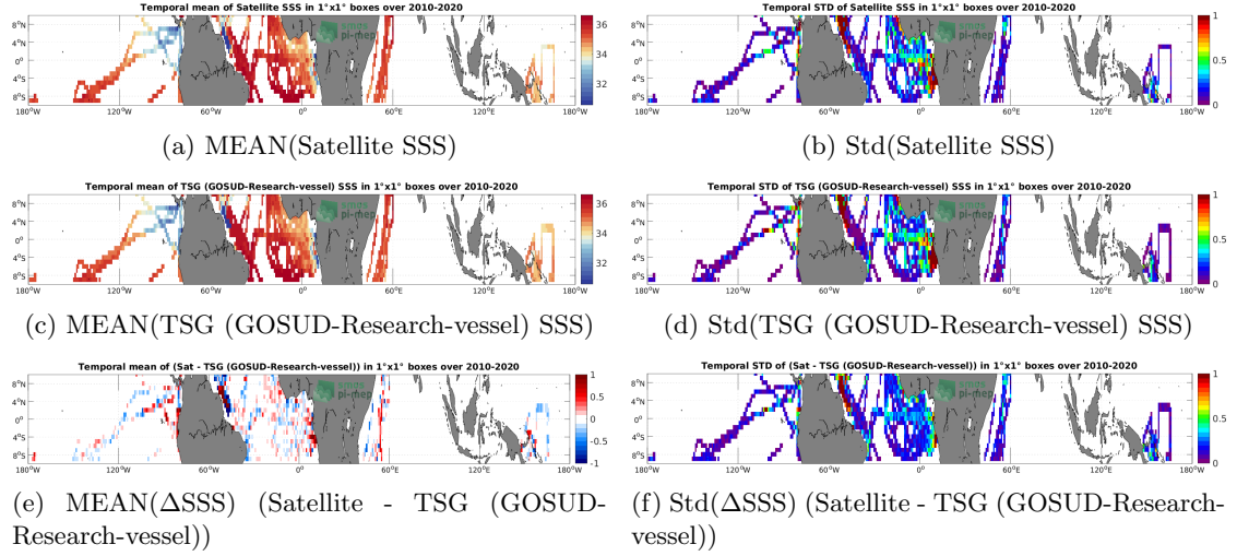
Figure 6: Temporal mean (left) and Std (right) of SSS from SMOS SSS L3 v8 - 9 Days (CATDS-CECOS-LOCEAN) (top), TSG (GOSUD-Research-vessel) (middle), and of \Delta SSS (Satellite - TSG (GOSUD-Research-vessel)). Only match-up pairs are used to generate these maps.
