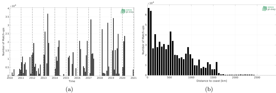
Figure 1: Number of match-ups between TSG (GOSUD-Research-vessel) and SMOS SSS L3 v8 - 9 Days (CATDS-CECOS-LOCEAN) SSS as a function of time (a) and as function of the distance to coast (b) over the Equatorial Ocean 10N-10S Pi-MEP region and for the full satellite product period.
