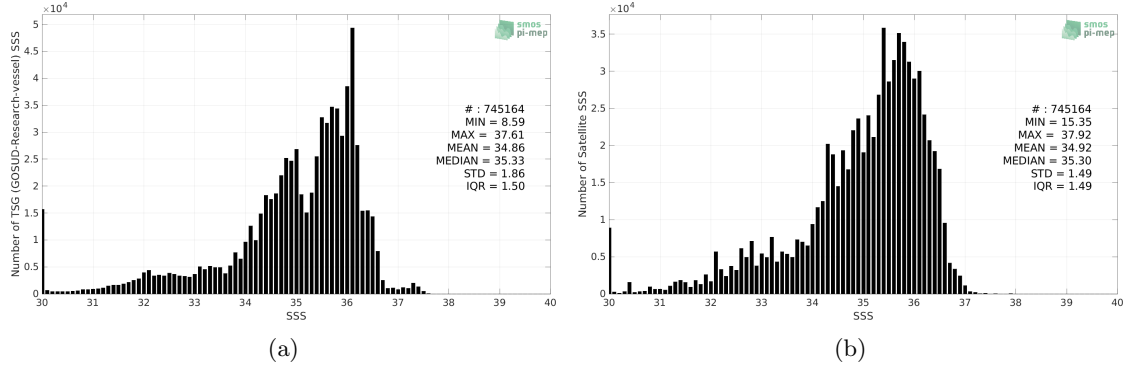
Figure 2: Histograms of SSS from TSG (GOSUD-Research-vessel) (a) and SMOS SSS L3 v8 - 9 Days (CATDS-CECOS-LOCEAN) (b) considering all match-up pairs per bins of 0.1 over the Equatorial Ocean 10N-10S Pi-MEP region and for the full satellite product period.
