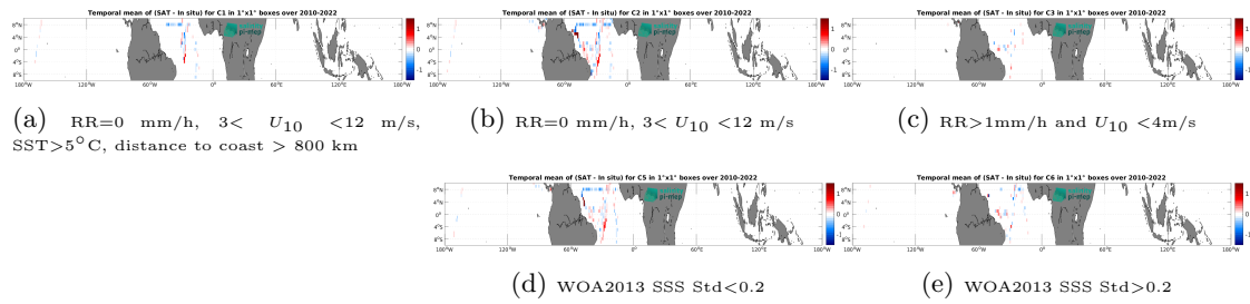
Figure 12: Temporal mean gridded over spatial boxes of size 1^\circ \times 1^\circ of \Delta\text{SSS} (SMOS SSS L3 v8 - 9 Days (CATDS-CEC-LOCEAN) - TSG (CSIC-UTM)) for 5 different subdatasets corresponding to:RR=0 mm/h, 3 < U_{10} < 12 m/s, SST >5^\circ\text{C} , distance to coast > 800 km (a), RR=0 mm/h, 3 < U_{10} < 12 m/s (b), RR >1 mm/h and U_{10} < 4 m/s (c), WOA2013 SSS Std <0.2 (d), WOA2013 SSS Std >0.2 (e).
