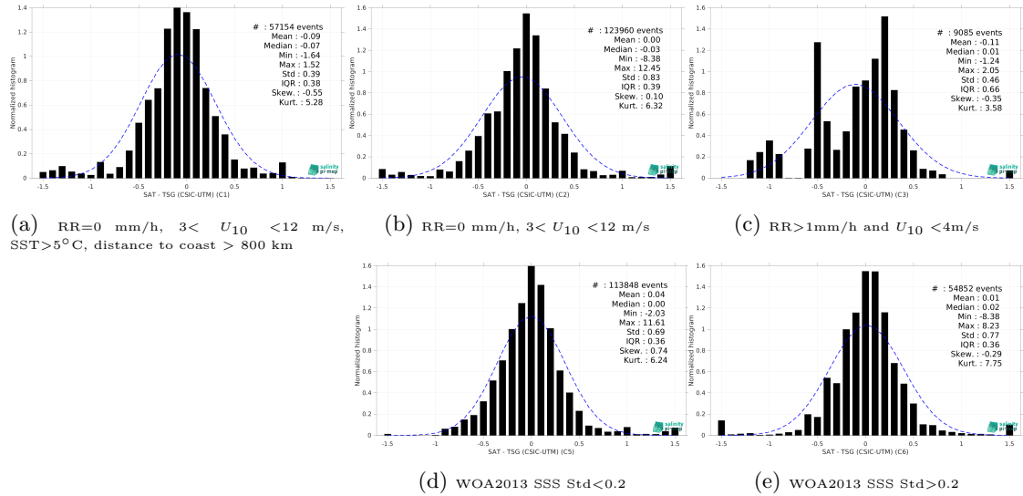
Figure 13: Normalized histogram of \Delta\text{SSS} (SMOS SSS L3 v8 - 9 Days (CATDS-CEC-LOCEAN) - TSG (CSIC-UTM)) for 5 different subdatasets corresponding to: RR=0 mm/h, 3 < U_{10} < 12 m/s, SST >5^\circ\text{C} , distance to coast > 800 km (a), RR=0 mm/h, 3 < U_{10} < 12 m/s (b), RR >1 mm/h and U_{10} < 4 m/s (c), WOA2013 SSS Std <0.2 (d), WOA2013 SSS Std >0.2 (e).
