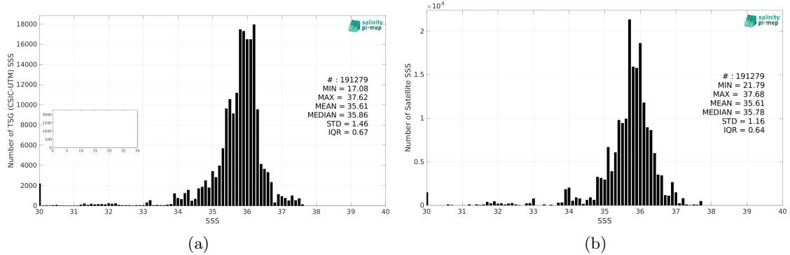
Figure 2: Histograms of SSS from TSG (CSIC-UTM) (a) and SMOS SSS L3 v8 - 9 Days (CATDS-CEC-LOCEAN) (b) considering all match-up pairs per bins of 0.1 over the Equatorial Ocean 10N-10S Pi-MEP region and for the full satellite product period.
