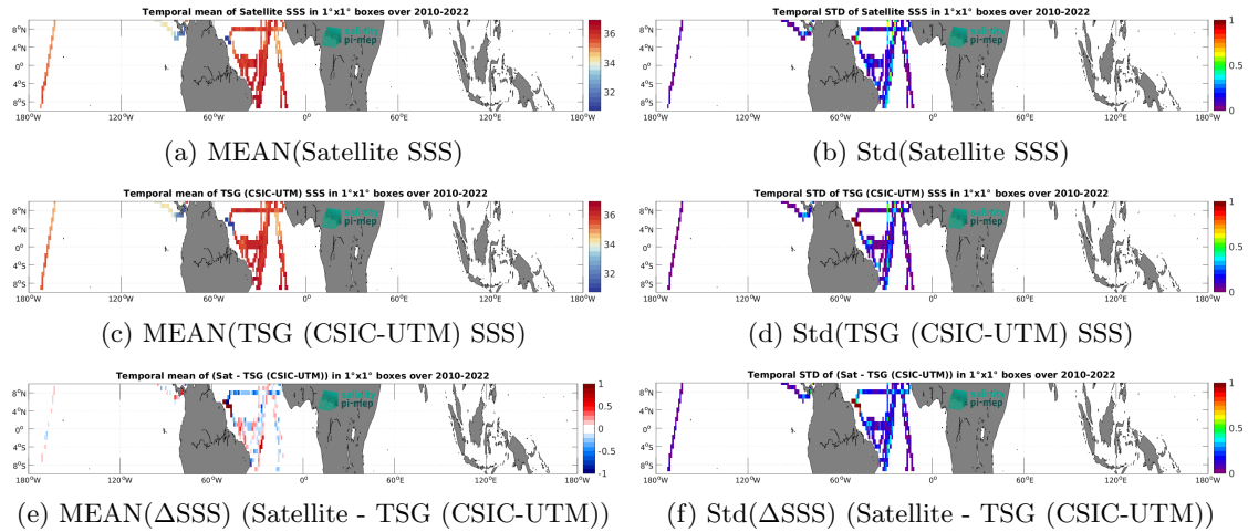
Figure 6: Temporal mean (left) and Std (right) of SSS from SMOS SSS L3 v8 - 9 Days (CATDS-CEC-LOCEAN) (top), TSG (CSIC-UTM) (middle), and of \Delta SSS (Satellite - TSG (CSIC-UTM)). Only match-up pairs are used to generate these maps.
