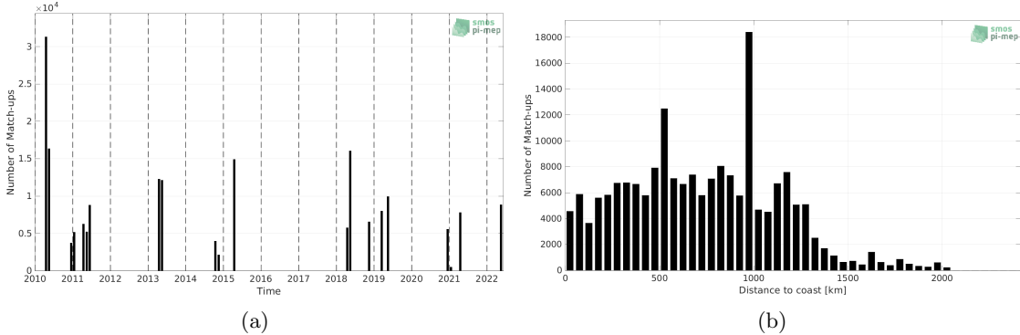
Figure 1: Number of match-ups between TSG (CSIC-UTM) and SMOS SSS L3 v8 - 9 Days (CATDS-CECOS-LOCEAN) SSS as a function of time (a) and as function of the distance to coast (b) over the Equatorial Ocean 10N-10S Pi-MEP region and for the full satellite product period.
