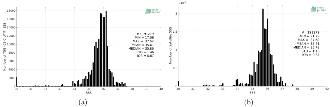
Figure 2: Histograms of SSS from TSG (CSIC-UTM) (a) and SMOS SSS L3 v8 - 9 Days (CATDS-CECOS-LOCEAN) (b) considering all match-up pairs per bins of 0.1 over the Equatorial Ocean 10N-10S Pi-MEP region and for the full satellite product period.
