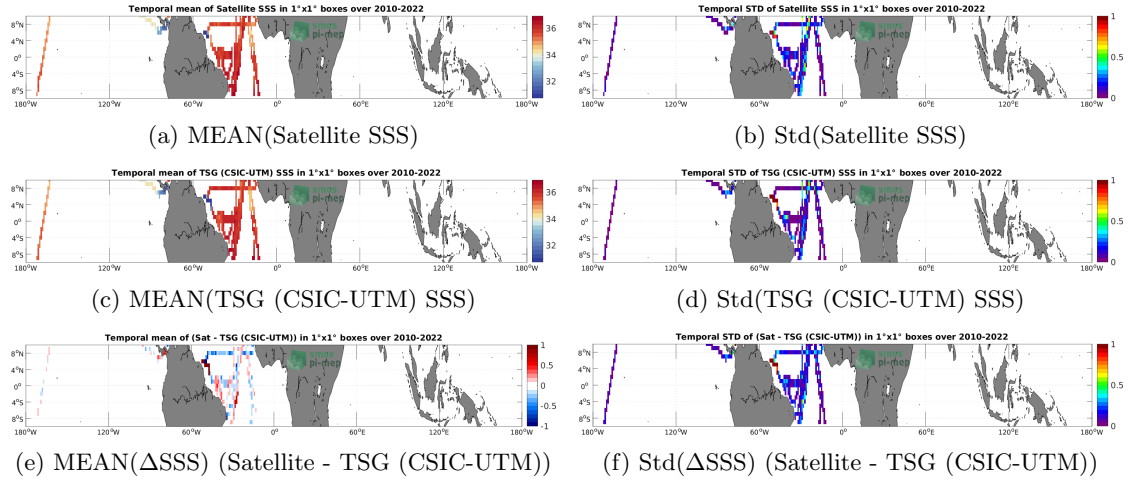
Figure 6: Temporal mean (left) and Std (right) of SSS from SMOS SSS L3 v8 - 9 Days (CATDS-CECOS-LOCEAN) (top), TSG (CSIC-UTM) (middle), and of \Delta SSS (Satellite - TSG (CSIC-UTM)). Only match-up pairs are used to generate these maps.
