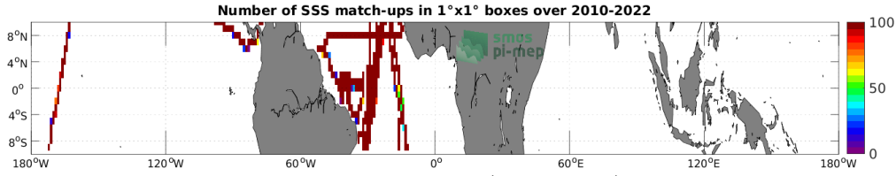
Figure 4: Number of SSS match-ups between TSG (CSIC-UTM) SSS and the SMOS SSS L3 v8 - 9 Days (CATDS-CECOS-LOCEAN) SSS product for the Equatorial Ocean 10N-10S Pi-MEP region over 1^\circ \times 1^\circ boxes and for the full satellite product period.
