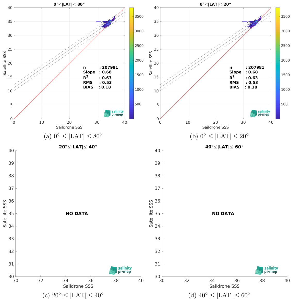
Figure 9: Contour maps of the concentration of SMOS SSS L3 v8 - 9 Days (CATDS-CEC-LOCEAN) SSS (y-axis) versus Saildrone SSS (x-axis) at match-up pairs for different latitude bands. For each plot, the red line shows x=y . The black thin and dashed lines indicate a linear fit through the data cloud and the \pm 95\% confidence levels, respectively. The number match-up pairs n , the slope and R^2 coefficient of the linear fit, the root mean square (RMS) and the mean bias between satellite and in situ data are indicated for each latitude band in each plots.
