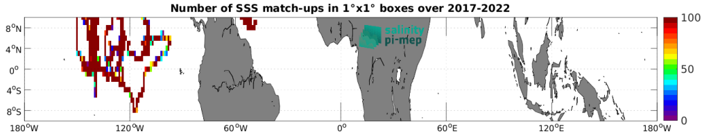
Figure 4: Number of SSS match-ups between Saildrone SSS and the SMOS SSS L3 v8 - 9 Days (CATDS-CEC-LOCEAN) SSS product for the Equatorial Ocean 10N-10S Pi-MEP region over 1^\circ \times 1^\circ boxes and for the full satellite product period.
