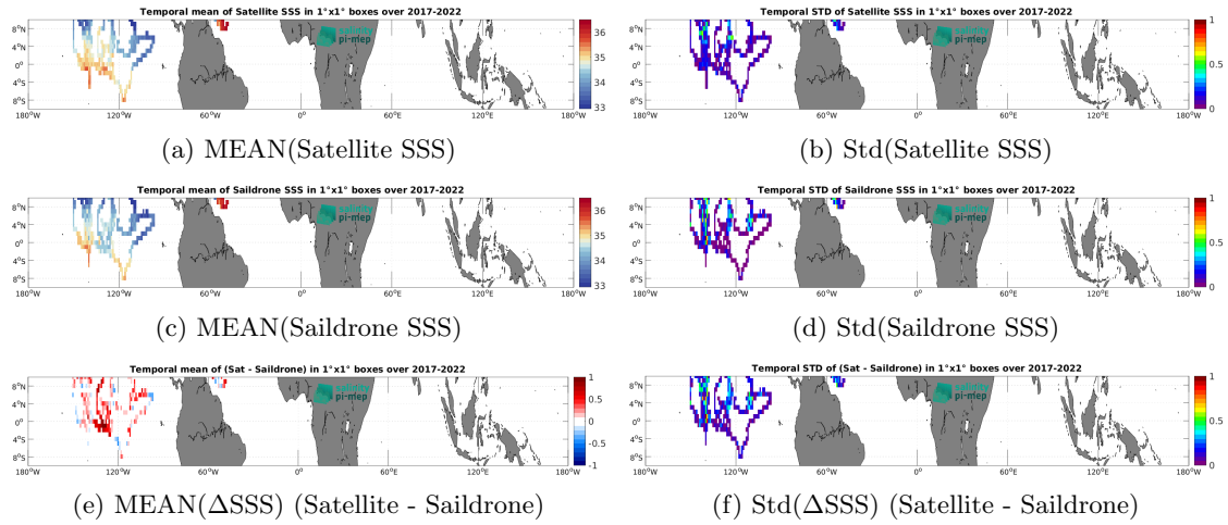
Figure 6: Temporal mean (left) and Std (right) of SSS from SMOS SSS L3 v8 - 9 Days (CATDS-CEC-LOCEAN) (top), Saildrone (middle), and of \Delta SSS (Satellite - Saildrone). Only match-up pairs are used to generate these maps.
