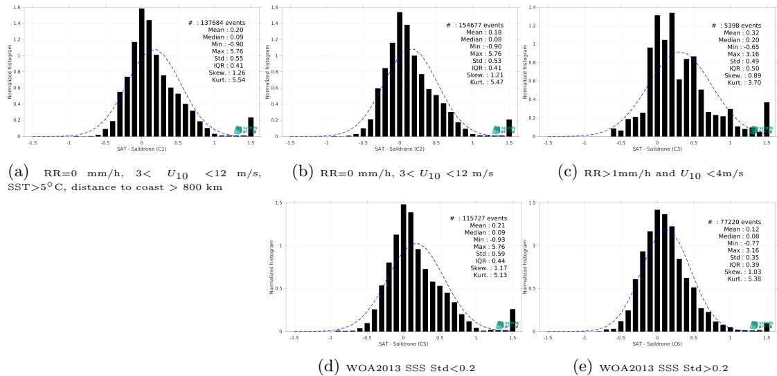
Figure 13: Normalized histogram of \Delta SSS (SMOS SSS L3 v8 - 9 Days (CATDS-CEC-LOCEAN) - Saildrone) for 5 different subdatasets corresponding to: RR=0 mm/h, 3 < U_{10} < 12 m/s, SST >5^\circ\text{C} , distance to coast > 800 km (a), RR=0 mm/h, 3 < U_{10} < 12 m/s (b), RR >1 mm/h and U_{10} < 4 m/s (c), WOA2013 SSS Std <0.2 (d), WOA2013 SSS Std >0.2 (e).
