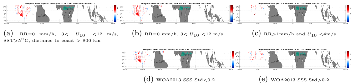
Figure 12: Temporal mean gridded over spatial boxes of size 1^\circ \times 1^\circ of \Delta SSS (SMOS SSS L3 v8 - 9 Days (CATDS-CEC-LOCEAN) - Saildrone) for 5 different subdatasets corresponding to: RR=0 mm/h, 3 < U_{10} < 12 m/s, SST >5^\circ\text{C} , distance to coast > 800 km (a), RR=0 mm/h, 3 < U_{10} < 12 m/s (b), RR >1 mm/h and U_{10} < 4 m/s (c), WOA2013 SSS Std <0.2 (d), WOA2013 SSS Std >0.2 (e).
