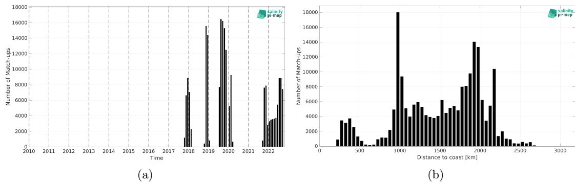
Figure 1: Number of match-ups between Saildrone and SMOS SSS L3 v8 - 9 Days (CATDS-CEC-LOCEAN) SSS as a function of time (a) and as function of the distance to coast (b) over the Equatorial Ocean 10N-10S Pi-MEP region and for the full satellite product period.
