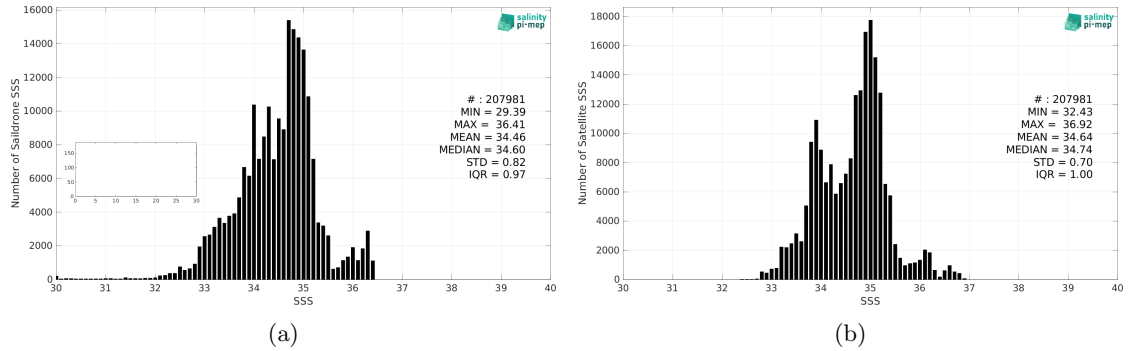
Figure 2: Histograms of SSS from Saildrone (a) and SMOS SSS L3 v8 - 9 Days (CATDS-CEC-LOCEAN) (b) considering all match-up pairs per bins of 0.1 over the Equatorial Ocean 10N-10S Pi-MEP region and for the full satellite product period.
