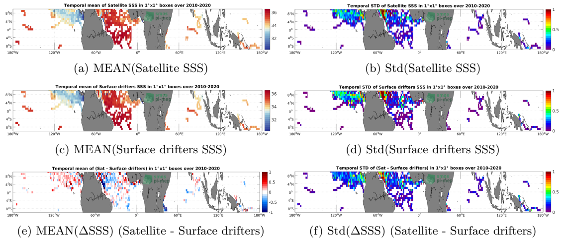
Figure 5: Temporal mean (left) and Std (right) of SSS from SMOS SSS L3 v8 - 9 Days (CATDS-CECOS-LOCEAN) (top), Surface drifters (middle), and of \Delta SSS (Satellite - Surface drifters). Only match-up pairs are used to generate these maps.
