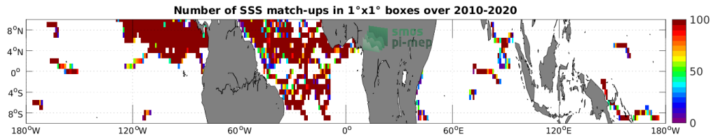
Figure 3: Number of SSS match-ups between Surface drifters SSS and the SMOS SSS L3 v8 - 9 Days (CATDS-CECOS-LOCEAN) SSS product for the Equatorial Ocean 10N-10S Pi-MEP region over 1^\circ \times 1^\circ boxes and for the full satellite product period.
