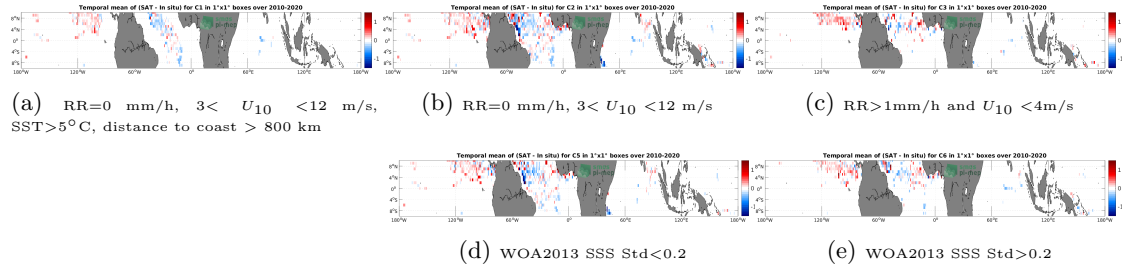
Figure 11: Temporal mean gridded over spatial boxes of size 1^{\circ}\times 1^{\circ} of \Delta\text{SSS} (SMOS SSS L3 v8 - 9 Days (CATDS-CECOS-LOCEAN) - Surface drifters) for 5 different subdatasets corresponding to:RR=0 mm/h, 3 < U_{10} < 12 m/s, SST >5^{\circ}\text{C} , distance to coast > 800 km (a), RR=0 mm/h, 3 < U_{10} < 12 m/s (b), RR >1 mm/h and U_{10} < 4 m/s (c), WOA2013 SSS Std <0.2 (d), WOA2013 SSS Std >0.2 (e).
