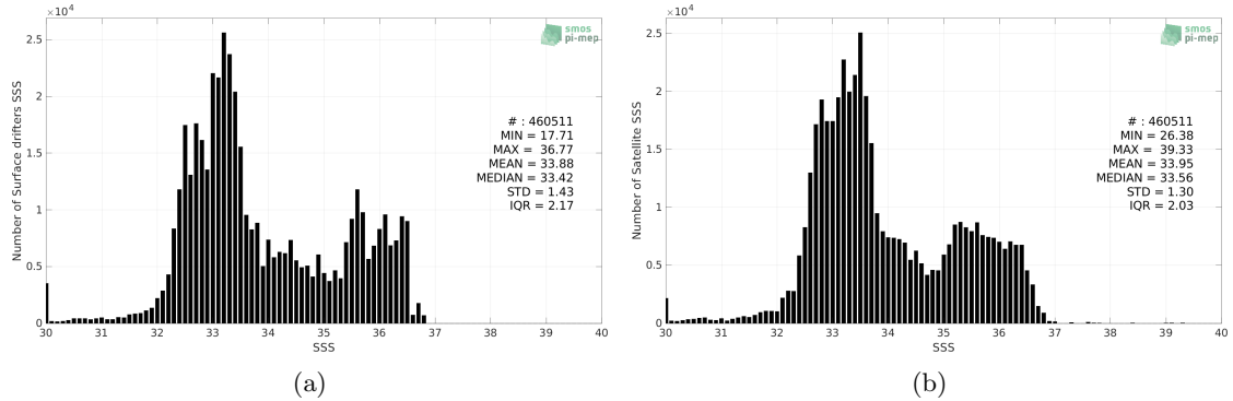
Figure 2: Histograms of SSS from Surface drifters (a) and SMOS SSS L3 v8 - 9 Days (CATDS-CECOS-LOCEAN) (b) considering all match-up pairs per bins of 0.1 over the Equatorial Ocean 10N-10S Pi-MEP region and for the full satellite product period.
