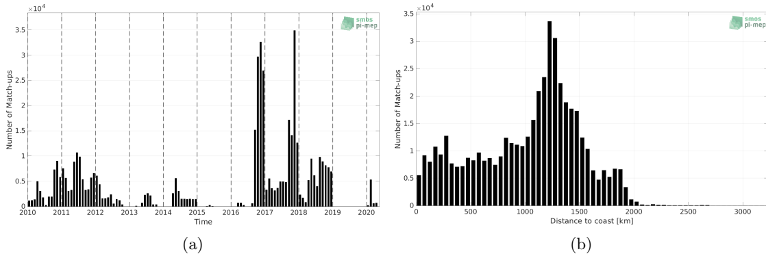
Figure 1: Number of match-ups between Surface drifters and SMOS SSS L3 v8 - 9 Days (CATDS-CECOS-LOCEAN) SSS as a function of time (a) and as function of the distance to coast (b) over the Equatorial Ocean 10N-10S Pi-MEP region and for the full satellite product period.
