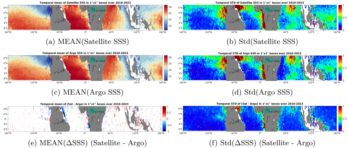
Figure 6: Temporal mean (left) and Std (right) of SSS from SMOS SSS L3 v8 - 9 Days (CATDS-CEC-LOCEAN) (top), Argo (middle), and of \Delta SSS (Satellite - Argo). Only match-up pairs are used to generate these maps.
