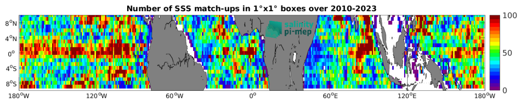
Figure 4: Number of SSS match-ups between Argo SSS and the SMOS SSS L3 v8 - 9 Days (CATDS-CEC-LOCEAN) SSS product for the Equatorial Ocean 10N-10S Pi-MEP region over 1^\circ \times 1^\circ boxes and for the full satellite product period.
