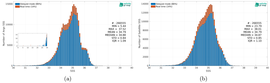
Figure 2: Histograms of SSS from Argo (a) and SMOS SSS L3 v8 - 9 Days (CATDS-CEC-LOCEAN) (b) considering all match-up pairs per bins of 0.1 over the Equatorial Ocean 10N-10S Pi-MEP region and for the full satellite product period.
