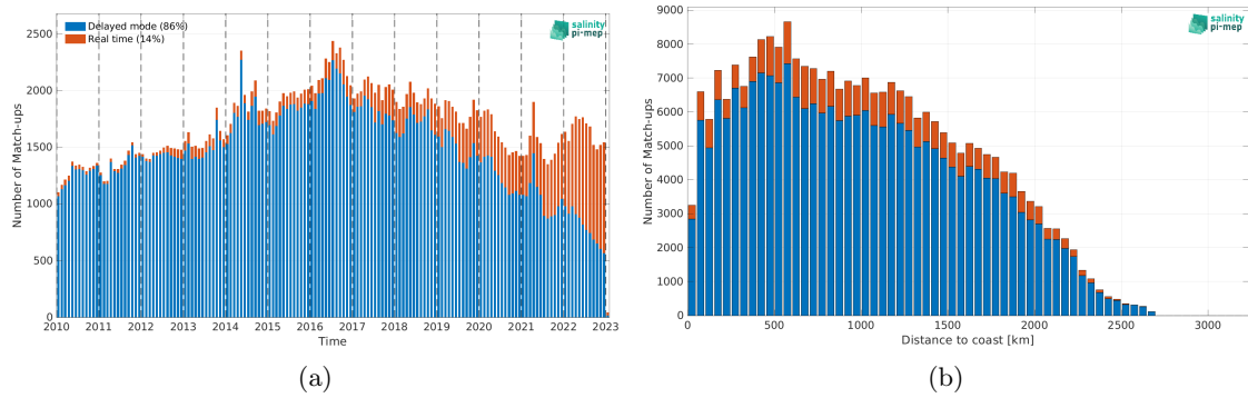
Figure 1: Number of match-ups between Argo and SMOS SSS L3 v8 - 9 Days (CATDS-CEC-LOCEAN) SSS as a function of time (a) and as function of the distance to coast (b) over the Equatorial Ocean 10N-10S Pi-MEP region and for the full satellite product period.
