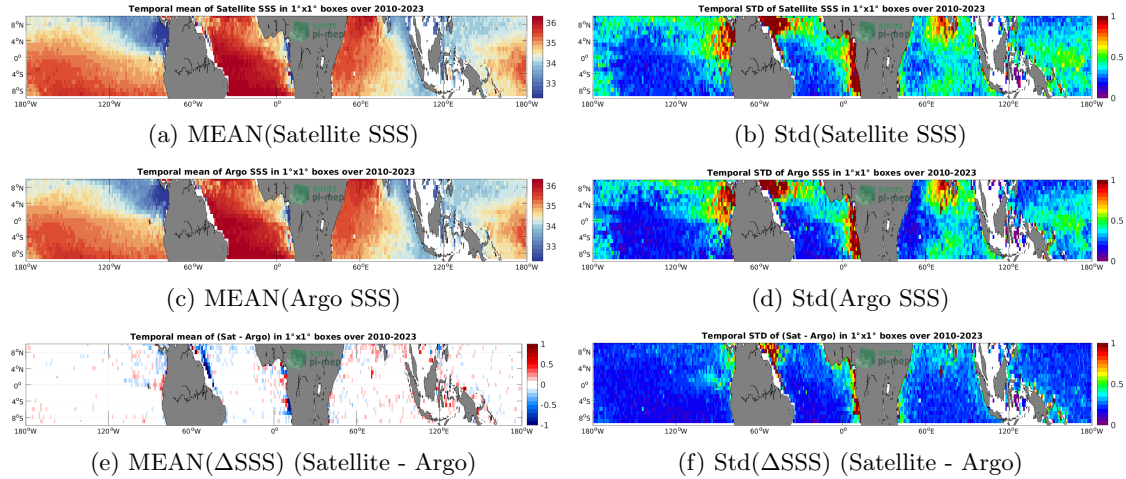
Figure 6: Temporal mean (left) and Std (right) of SSS from SMOS SSS L3 v8 - 9 Days (CATDS-CECOS-LOCEAN) (top), Argo (middle), and of \Delta SSS (Satellite - Argo). Only match-up pairs are used to generate these maps.
