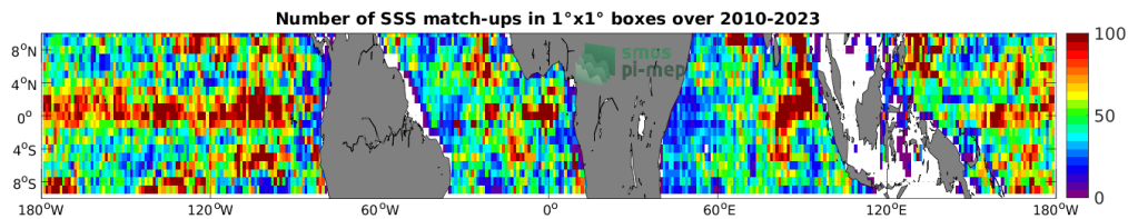
Figure 4: Number of SSS match-ups between Argo SSS and the SMOS SSS L3 v8 - 9 Days (CATDS-CECOS-LOCEAN) SSS product for the Equatorial Ocean 10N-10S Pi-MEP region over 1^\circ \times 1^\circ boxes and for the full satellite product period.
