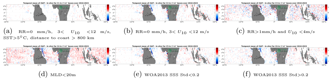
Figure 12: Temporal mean gridded over spatial boxes of size 1^\circ \times 1^\circ of \Delta SSS (SMOS SSS L3 v8 - 9 Days (CATDS-CECOS-LOCEAN) - Argo) for 6 different subdatasets corresponding to:RR=0 mm/h, 3 < U_{10} < 12 m/s, SST >5^\circ C, distance to coast > 800 km (a), RR=0 mm/h, 3 < U_{10} < 12 m/s (b), RR >1 mm/h and U_{10} < 4 m/s (c),MLD <20 m (d),WOA2013 SSS Std <0.2 (e),WOA2013 SSS Std >0.2 (f).
