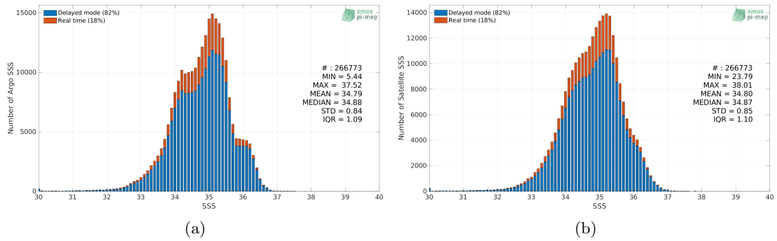
Figure 2: Histograms of SSS from Argo (a) and SMOS SSS L3 v8 - 9 Days (CATDS-CECOS-LOCEAN) (b) considering all match-up pairs per bins of 0.1 over the Equatorial Ocean 10N-10S Pi-MEP region and for the full satellite product period.
