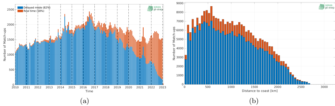
Figure 1: Number of match-ups between Argo and SMOS SSS L3 v8 - 9 Days (CATDS-CECOS-LOCEAN) SSS as a function of time (a) and as function of the distance to coast (b) over the Equatorial Ocean 10N-10S Pi-MEP region and for the full satellite product period.
