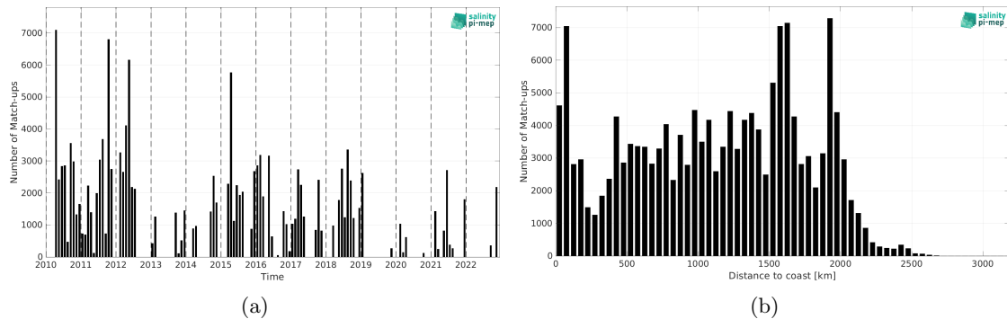
Figure 1: Number of match-ups between TSG (SAMOS) and SMOS SSS L3 v8 - 18 Days (CATDS-CEC-LOCEAN) SSS as a function of time (a) and as function of the distance to coast (b) over the Equatorial Ocean 10N-10S Pi-MEP region and for the full satellite product period.
