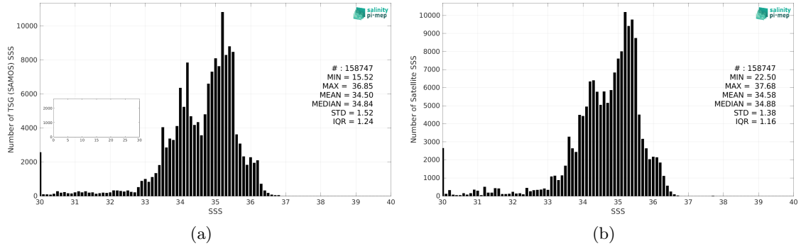
Figure 2: Histograms of SSS from TSG (SAMOS) (a) and SMOS SSS L3 v8 - 18 Days (CATDS-CEC-LOCEAN) (b) considering all match-up pairs per bins of 0.1 over the Equatorial Ocean 10N-10S Pi-MEP region and for the full satellite product period.
