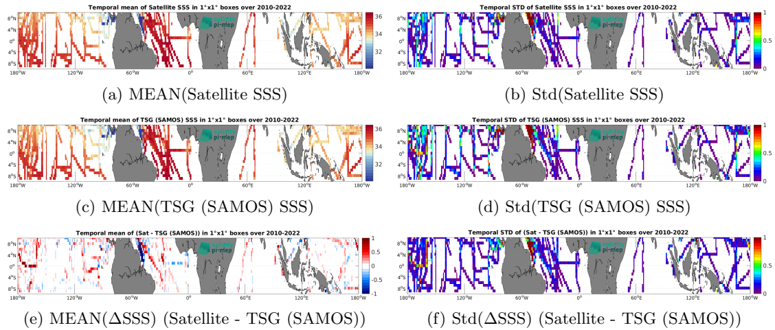
Figure 6: Temporal mean (left) and Std (right) of SSS from SMOS SSS L3 v8 - 18 Days (CATDS-CEC-LOCEAN) (top), TSG (SAMOS) (middle), and of \Delta SSS (Satellite - TSG (SAMOS)). Only match-up pairs are used to generate these maps.
