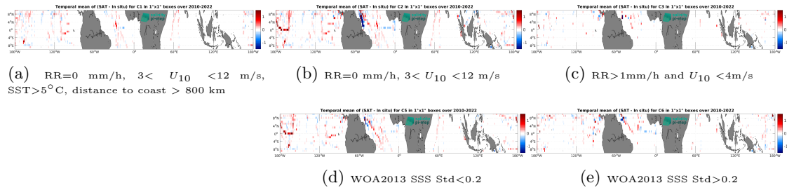
Figure 12: Temporal mean gridded over spatial boxes of size 1^\circ \times 1^\circ of \Delta\text{SSS} (SMOS SSS L3 v8 - 18 Days (CATDS-CEC-LOCEAN) - TSG (SAMOS)) for 5 different subdatasets corresponding to: RR=0 mm/h, 3 < U_{10} < 12 m/s, SST >5^\circ\text{C} , distance to coast > 800 km (a), RR=0 mm/h, 3 < U_{10} < 12 m/s (b), RR >1 mm/h and U_{10} < 4 m/s (c), WOA2013 SSS Std <0.2 (d), WOA2013 SSS Std >0.2 (e).
