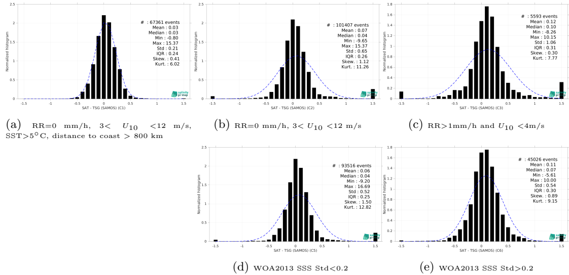
Figure 13: Normalized histogram of \Delta\text{SSS} (SMOS SSS L3 v8 - 18 Days (CATDS-CEC-LOCEAN) - TSG (SAMOS)) for 5 different subdatasets corresponding to: RR=0 mm/h, 3 < U_{10} < 12 m/s, SST >5^\circ\text{C} , distance to coast > 800 km (a), RR=0 mm/h, 3 < U_{10} < 12 m/s (b), RR >1 mm/h and U_{10} < 4 m/s (c), WOA2013 SSS Std <0.2 (d), WOA2013 SSS Std >0.2 (e).
