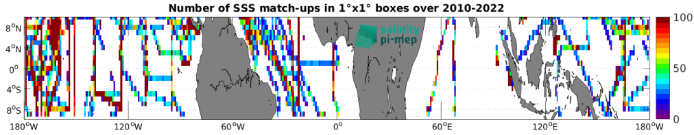
Figure 4: Number of SSS match-ups between TSG (SAMOS) SSS and the SMOS SSS L3 v8 - 18 Days (CATDS-CEC-LOCEAN) SSS product for the Equatorial Ocean 10N-10S Pi-MEP region over 1^\circ \times 1^\circ boxes and for the full satellite product period.
