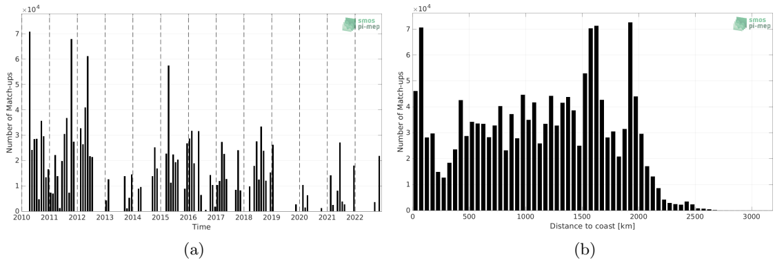
Figure 1: Number of match-ups between TSG (SAMOS) and SMOS SSS L3 v8 - 18 Days (CATDS-CECOS-LOCEAN) SSS as a function of time (a) and as function of the distance to coast (b) over the Equatorial Ocean 10N-10S Pi-MEP region and for the full satellite product period.
