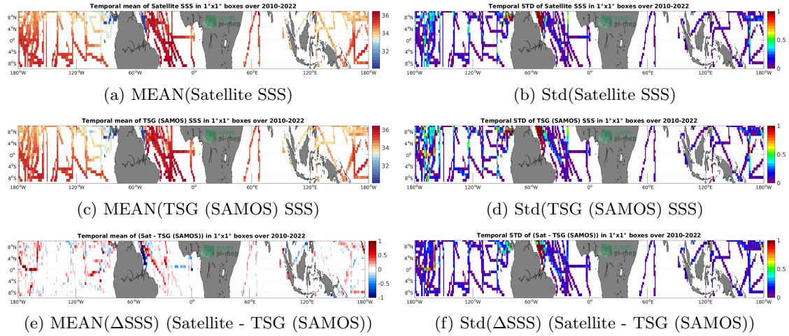
Figure 6: Temporal mean (left) and Std (right) of SSS from SMOS SSS L3 v8 - 18 Days (CATDS-CECOS-LOCEAN) (top), TSG (SAMOS) ( in situ ) (middle), and of \Delta SSS (Satellite - TSG (SAMOS)). Only match-up pairs are used to generate these maps.
