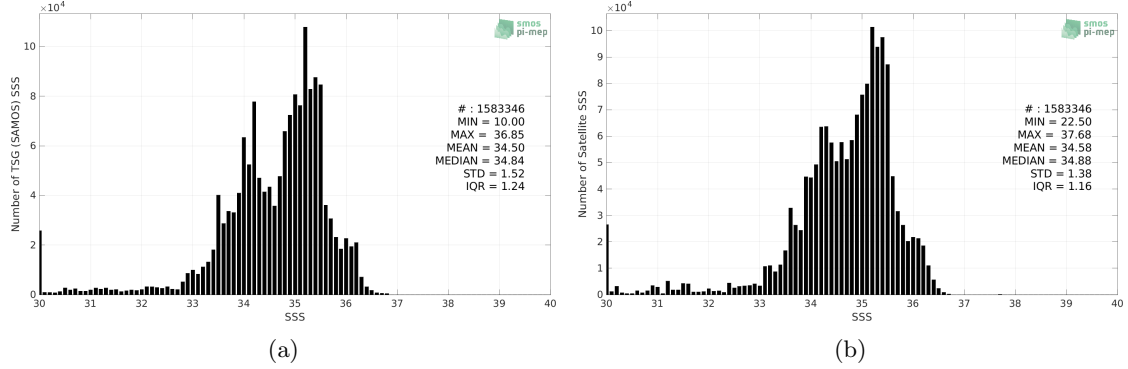
Figure 2: Histograms of SSS from TSG (SAMOS) (a) and SMOS SSS L3 v8 - 18 Days (CATDS-CECOS-LOCEAN) (b) considering all match-up pairs per bins of 0.1 over the Equatorial Ocean 10N-10S Pi-MEP region and for the full satellite product period.
