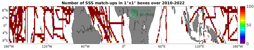
Figure 4: Number of SSS match-ups between TSG (SAMOS) SSS and the SMOS SSS L3 v8 - 18 Days (CATDS-CECOS-LOCEAN) SSS product for the Equatorial Ocean 10N-10S Pi-MEP region over 1^\circ \times 1^\circ boxes and for the full satellite product period.
