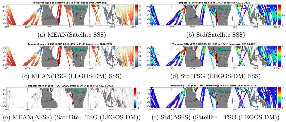
Figure 6: Temporal mean (left) and Std (right) of SSS from SMOS SSS L3 v8 - 18 Days (CATDS-CEC-LOCEAN) (top), TSG (LEGOS-DM) (middle), and of \Delta SSS (Satellite - TSG (LEGOS-DM)). Only match-up pairs are used to generate these maps.
