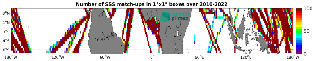
Figure 4: Number of SSS match-ups between TSG (LEGOS-DM) SSS and the SMOS SSS L3 v8 - 18 Days (CATDS-CEC-LOCEAN) SSS product for the Equatorial Ocean 10N-10S Pi-MEP region over 1^\circ \times 1^\circ boxes and for the full satellite product period.
