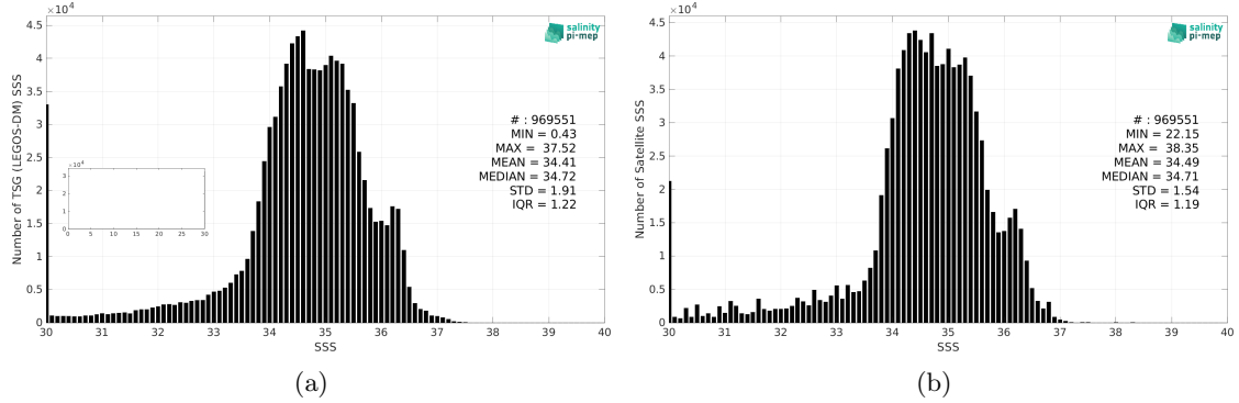
Figure 2: Histograms of SSS from TSG (LEGOS-DM) (a) and SMOS SSS L3 v8 - 18 Days (CATDS-CEC-LOCEAN) (b) considering all match-up pairs per bins of 0.1 over the Equatorial Ocean 10N-10S Pi-MEP region and for the full satellite product period.
