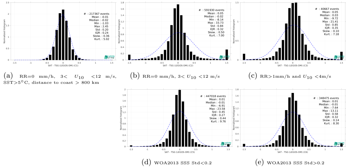
Figure 13: Normalized histogram of \Delta SSS (SMOS SSS L3 v8 - 18 Days (CATDS-CEC-LOCEAN) - TSG (LEGOS-DM)) for 5 different subdatasets corresponding to: RR=0 mm/h, 3 < U_{10} < 12 m/s, SST > 5^\circ C , distance to coast > 800 km (a), RR=0 mm/h, 3 < U_{10} < 12 m/s (b), RR > 1 mm/h and U_{10} < 4 m/s (c), WOA2013 SSS Std < 0.2 (d), WOA2013 SSS Std > 0.2 (e).
