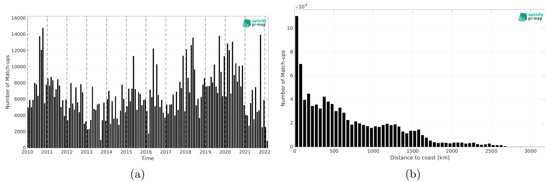
Figure 1: Number of match-ups between TSG (LEGOS-DM) and SMOS SSS L3 v8 - 18 Days (CATDS-CEC-LOCEAN) SSS as a function of time (a) and as function of the distance to coast (b) over the Equatorial Ocean 10N-10S Pi-MEP region and for the full satellite product period.
