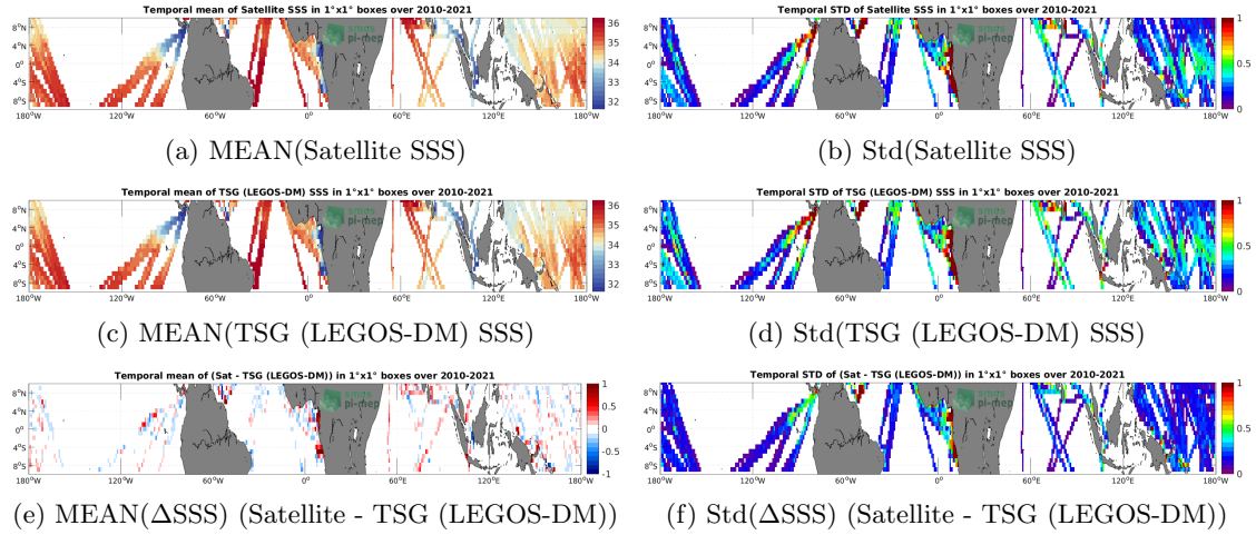
Figure 6: Temporal mean (left) and Std (right) of SSS from SMOS SSS L3 v8 - 18 Days (CATDS-CECOS-LOCEAN) (top), TSG (LEGOS-DM) (middle), and of \Delta SSS (Satellite - TSG (LEGOS-DM)). Only match-up pairs are used to generate these maps.
