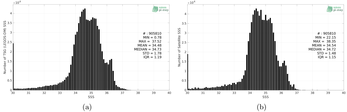
Figure 2: Histograms of SSS from TSG (LEGOS-DM) (a) and SMOS SSS L3 v8 - 18 Days (CATDS-CECOS-LOCEAN) (b) considering all match-up pairs per bins of 0.1 over the Equatorial Ocean 10N-10S Pi-MEP region and for the full satellite product period.
