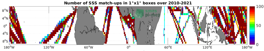
Figure 4: Number of SSS match-ups between TSG (LEGOS-DM) SSS and the SMOS SSS L3 v8 - 18 Days (CATDS-CECOS-LOCEAN) SSS product for the Equatorial Ocean 10N-10S Pi-MEP region over 1^\circ \times 1^\circ boxes and for the full satellite product period.
