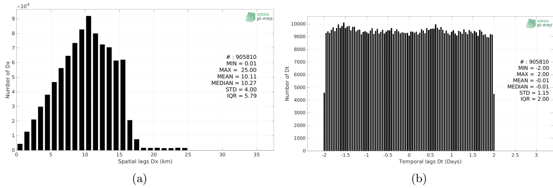
Figure 5: Histograms of the spatial (a) and temporal (b) lags between the location/time of the TSG (LEGOS-DM) measurement and the date of the corresponding SMOS SSS L3 v8 - 18 Days (CATDS-CECOS-LOCEAN) SSS pixel.
