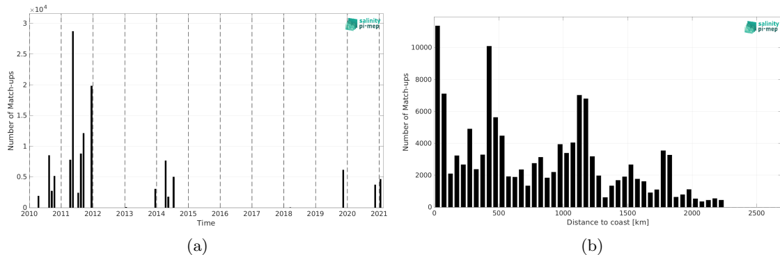
Figure 1: Number of match-ups between TSG (GOSUD-Sailing-ship) and SMOS SSS L3 v8 - 18 Days (CATDS-CEC-LOCEAN) SSS as a function of time (a) and as function of the distance to coast (b) over the Equatorial Ocean 10N-10S Pi-MEP region and for the full satellite product period.
