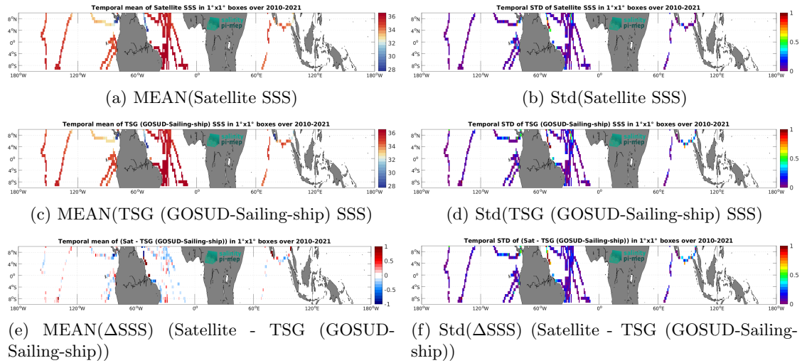
Figure 6: Temporal mean (left) and Std (right) of SSS from SMOS SSS L3 v8 - 18 Days (CATDS-CEC-LOCEAN) (top), TSG (GOSUD-Sailing-ship) (middle), and of \Delta SSS (Satellite - TSG (GOSUD-Sailing-ship)). Only match-up pairs are used to generate these maps.
