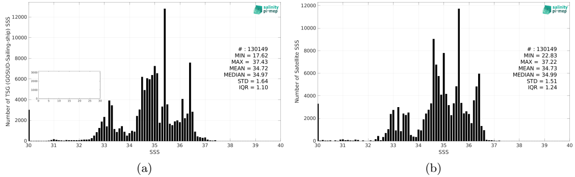
Figure 2: Histograms of SSS from TSG (GOSUD-Sailing-ship) (a) and SMOS SSS L3 v8 - 18 Days (CATDS-CEC-LOCEAN) (b) considering all match-up pairs per bins of 0.1 over the Equatorial Ocean 10N-10S Pi-MEP region and for the full satellite product period.
