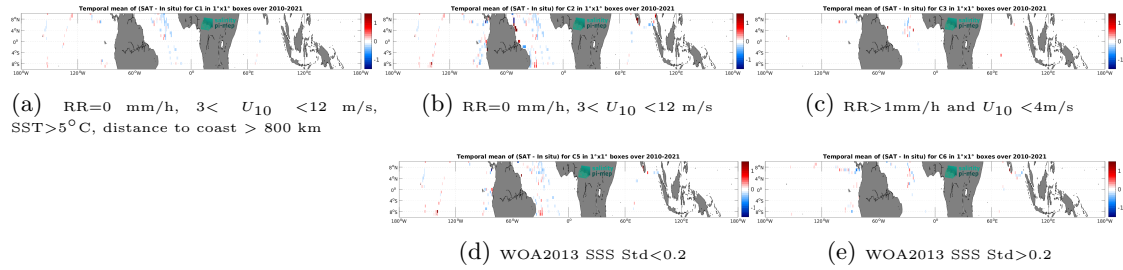
Figure 12: Temporal mean gridded over spatial boxes of size 1^{\circ}\times 1^{\circ} of \Delta SSS (SMOS SSS L3 v8 - 18 Days (CATDS-CEC-LOCEAN) - TSG (GOSUD-Sailing-ship)) for 5 different subdatasets corresponding to:RR=0 mm/h, 3 < U_{10} < 12 m/s, SST >5^{\circ}\text{C} , distance to coast > 800 km (a), RR=0 mm/h, 3 < U_{10} < 12 m/s (b), RR >1 mm/h and U_{10} < 4 m/s (c), WOA2013 SSS Std <0.2 (d), WOA2013 SSS Std >0.2 (e).
