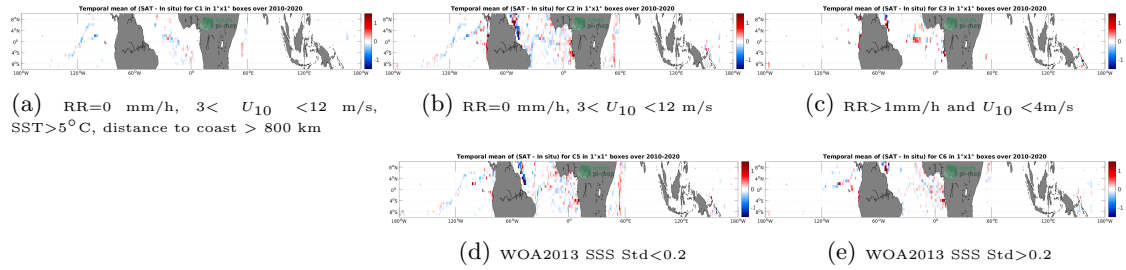
Figure 12: Temporal mean gridded over spatial boxes of size 1^{\circ}\times 1^{\circ} of \Delta SSS (SMOS SSS L3 v8 - 18 Days (CATDS-CECOS-LOCEAN) - TSG (GOSUD-Research-vessel)) for 5 different sub-datasets corresponding to:RR=0 mm/h, 3 < U_{10} < 12 m/s, SST >5^{\circ}\text{C} , distance to coast > 800 km (a), RR=0 mm/h, 3 < U_{10} < 12 m/s (b), RR >1 mm/h and U_{10} < 4 m/s (c), WOA2013 SSS Std <0.2 (d), WOA2013 SSS Std >0.2 (e).
