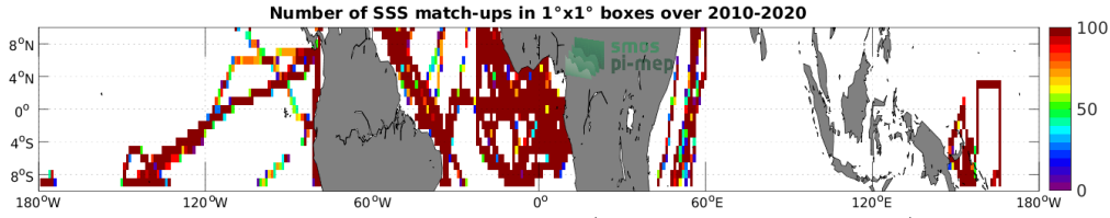
Figure 4: Number of SSS match-ups between TSG (GOSUD-Research-vessel) SSS and the SMOS SSS L3 v8 - 18 Days (CATDS-CECOS-LOCEAN) SSS product for the Equatorial Ocean 10N-10S Pi-MEP region over 1^\circ \times 1^\circ boxes and for the full satellite product period.
