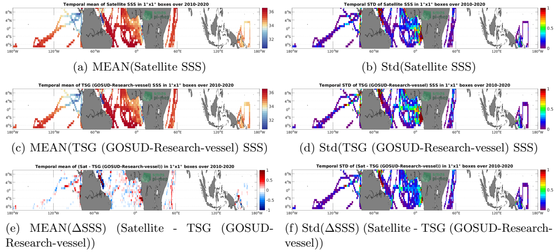
Figure 6: Temporal mean (left) and Std (right) of SSS from SMOS SSS L3 v8 - 18 Days (CATDS-CECOS-LOCEAN) (top), TSG (GOSUD-Research-vessel) (middle), and of \Delta SSS (Satellite - TSG (GOSUD-Research-vessel)). Only match-up pairs are used to generate these maps.
