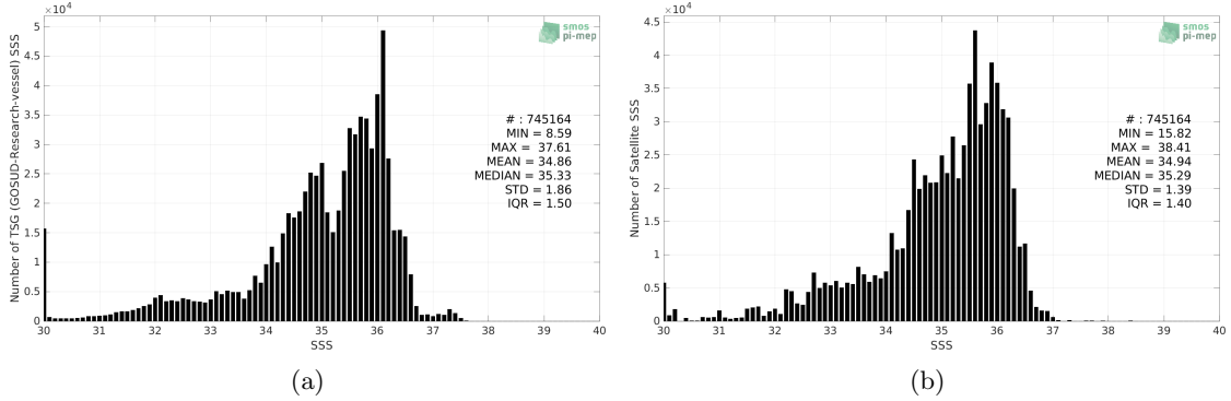
Figure 2: Histograms of SSS from TSG (GOSUD-Research-vessel) (a) and SMOS SSS L3 v8 - 18 Days (CATDS-CECOS-LOCEAN) (b) considering all match-up pairs per bins of 0.1 over the Equatorial Ocean 10N-10S Pi-MEP region and for the full satellite product period.
