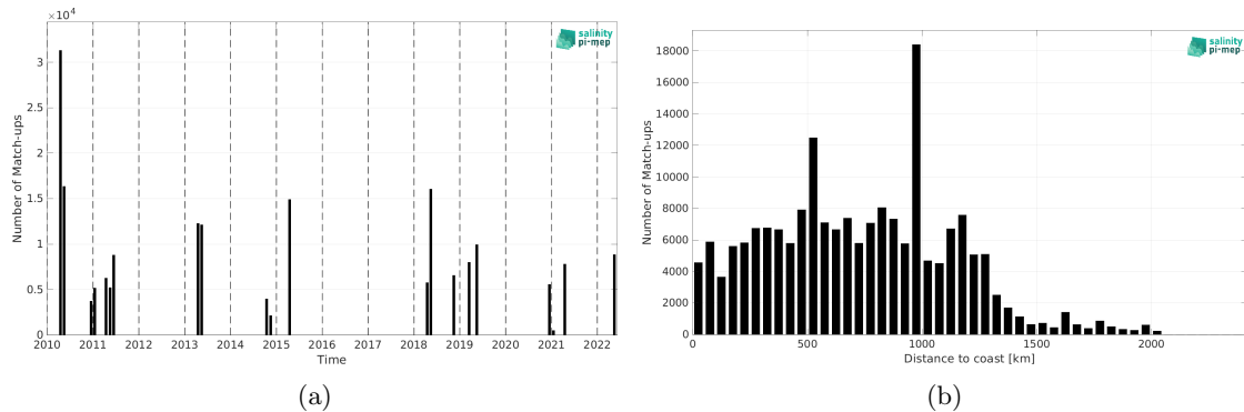
Figure 1: Number of match-ups between TSG (CSIC-UTM) and SMOS SSS L3 v8 - 18 Days (CATDS-CEC-LOCEAN) SSS as a function of time (a) and as function of the distance to coast (b) over the Equatorial Ocean 10N-10S Pi-MEP region and for the full satellite product period.
