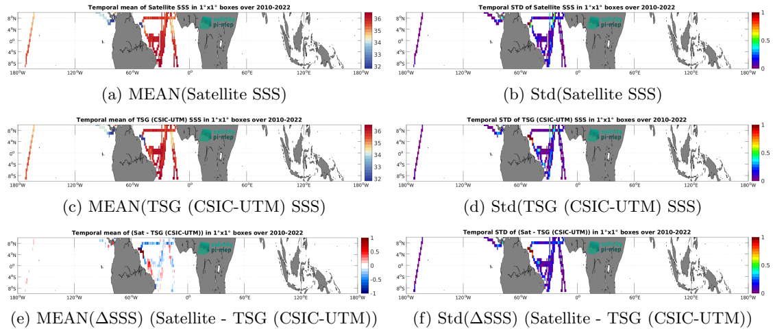
Figure 6: Temporal mean (left) and Std (right) of SSS from SMOS SSS L3 v8 - 18 Days (CATDS-CEC-LOCEAN) (top), TSG (CSIC-UTM) (middle), and of \Delta SSS (Satellite - TSG (CSIC-UTM)). Only match-up pairs are used to generate these maps.
