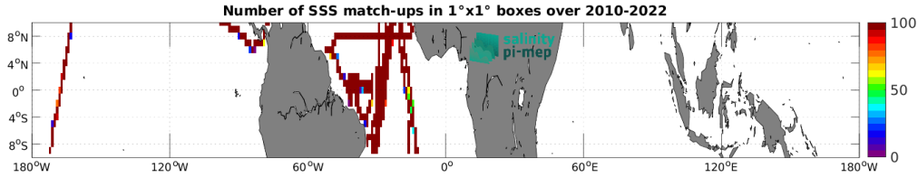
Figure 4: Number of SSS match-ups between TSG (CSIC-UTM) SSS and the SMOS SSS L3 v8 - 18 Days (CATDS-CEC-LOCEAN) SSS product for the Equatorial Ocean 10N-10S Pi-MEP region over 1^\circ \times 1^\circ boxes and for the full satellite product period.
