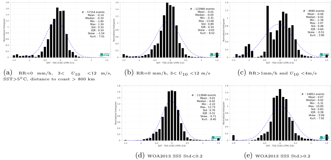
Figure 13: Normalized histogram of \Delta SSS (SMOS SSS L3 v8 - 18 Days (CATDS-CEC-LOCEAN) - TSG (CSIC-UTM)) for 5 different subdatasets corresponding to: RR=0 mm/h, 3 < U_{10} < 12 m/s, SST >5^\circ C, distance to coast > 800 km (a), RR=0 mm/h, 3 < U_{10} < 12 m/s (b), RR >1 mm/h and U_{10} < 4 m/s (c), WOA2013 SSS Std <0.2 (d), WOA2013 SSS Std >0.2 (e).
