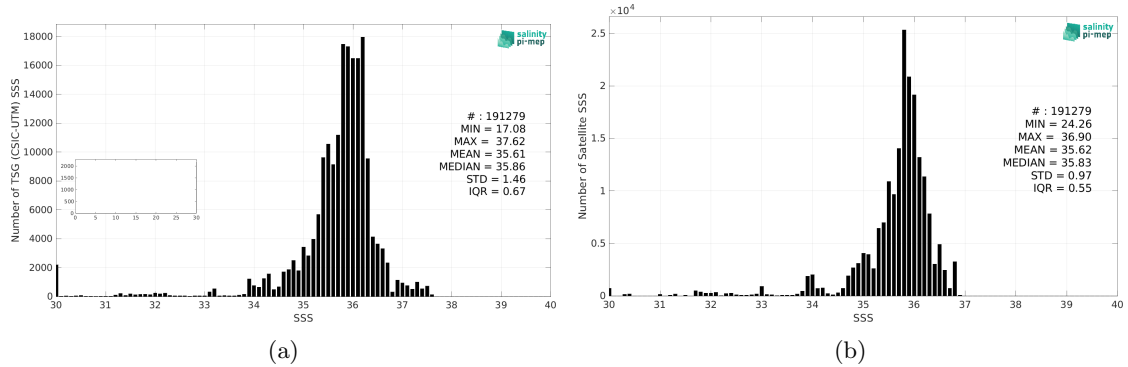
Figure 2: Histograms of SSS from TSG (CSIC-UTM) (a) and SMOS SSS L3 v8 - 18 Days (CATDS-CEC-LOCEAN) (b) considering all match-up pairs per bins of 0.1 over the Equatorial Ocean 10N-10S Pi-MEP region and for the full satellite product period.
