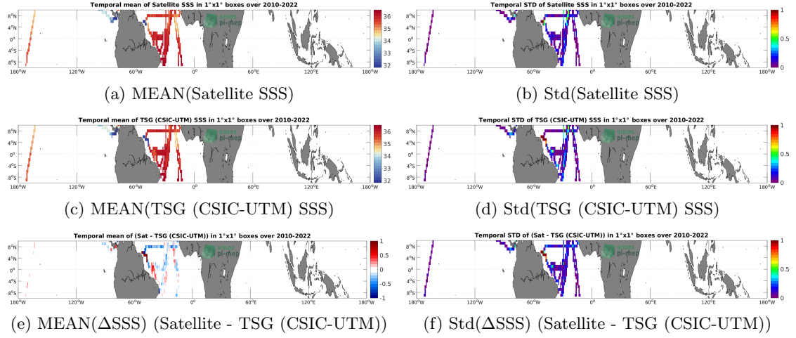
Figure 6: Temporal mean (left) and Std (right) of SSS from SMOS SSS L3 v8 - 18 Days (CATDS-CECOS-LOCEAN) (top), TSG (CSIC-UTM) (middle), and of \Delta SSS (Satellite - TSG (CSIC-UTM)). Only match-up pairs are used to generate these maps.
