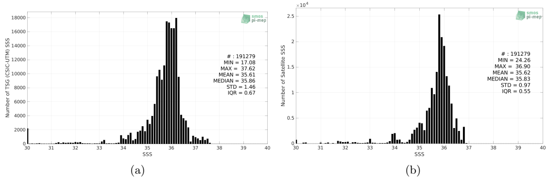
Figure 2: Histograms of SSS from TSG (CSIC-UTM) (a) and SMOS SSS L3 v8 - 18 Days (CATDS-CECOS-LOCEAN) (b) considering all match-up pairs per bins of 0.1 over the Equatorial Ocean 10N-10S Pi-MEP region and for the full satellite product period.
