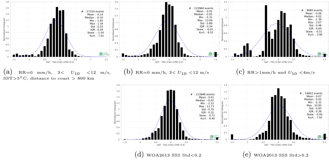
Figure 13: Normalized histogram of \Delta\text{SSS} (SMOS SSS L3 v8 - 18 Days (CATDS-CECOS-LOCEAN) - TSG (CSIC-UTM)) for 5 different subdatasets corresponding to: RR=0 mm/h, 3 < U_{10} < 12 m/s, SST>5°C, distance to coast > 800 km (a), RR=0 mm/h, 3 < U_{10} < 12 m/s (b), RR>1mm/h and U_{10} < 4 m/s (c), WOA2013 SSS Std<0.2 (d), WOA2013 SSS Std>0.2 (e).
