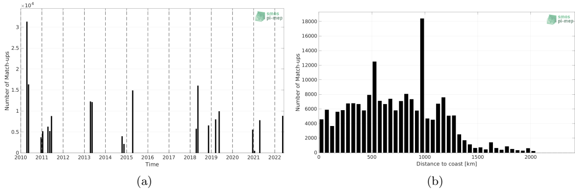
Figure 1: Number of match-ups between TSG (CSIC-UTM) and SMOS SSS L3 v8 - 18 Days (CATDS-CECOS-LOCEAN) SSS as a function of time (a) and as function of the distance to coast (b) over the Equatorial Ocean 10N-10S Pi-MEP region and for the full satellite product period.
