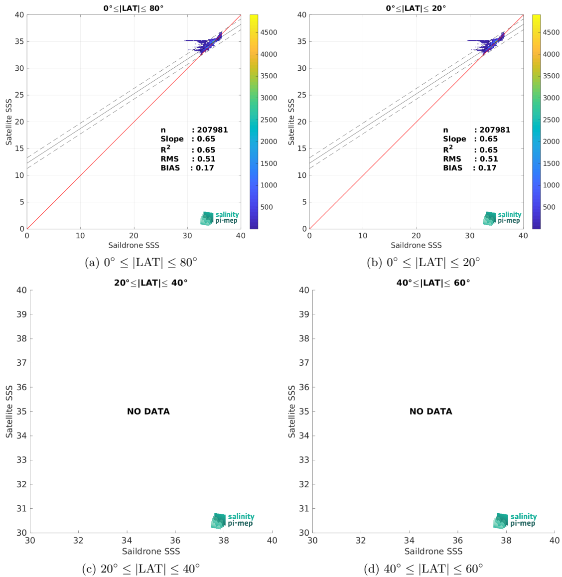
Figure 9: Contour maps of the concentration of SMOS SSS L3 v8 - 18 Days (CATDS-CEC-LOCEAN) SSS (y-axis) versus Saildrone SSS (x-axis) at match-up pairs for different latitude bands. For each plot, the red line shows x=y . The black thin and dashed lines indicate a linear fit through the data cloud and the \pm 95\% confidence levels, respectively. The number match-up pairs n , the slope and R^2 coefficient of the linear fit, the root mean square (RMS) and the mean bias between satellite and in situ data are indicated for each latitude band in each plots.
