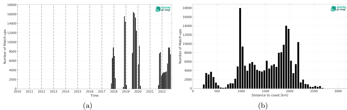
Figure 1: Number of match-ups between Saildrone and SMOS SSS L3 v8 - 18 Days (CATDS-CEC-LOCEAN) SSS as a function of time (a) and as function of the distance to coast (b) over the Equatorial Ocean 10N-10S Pi-MEP region and for the full satellite product period.
