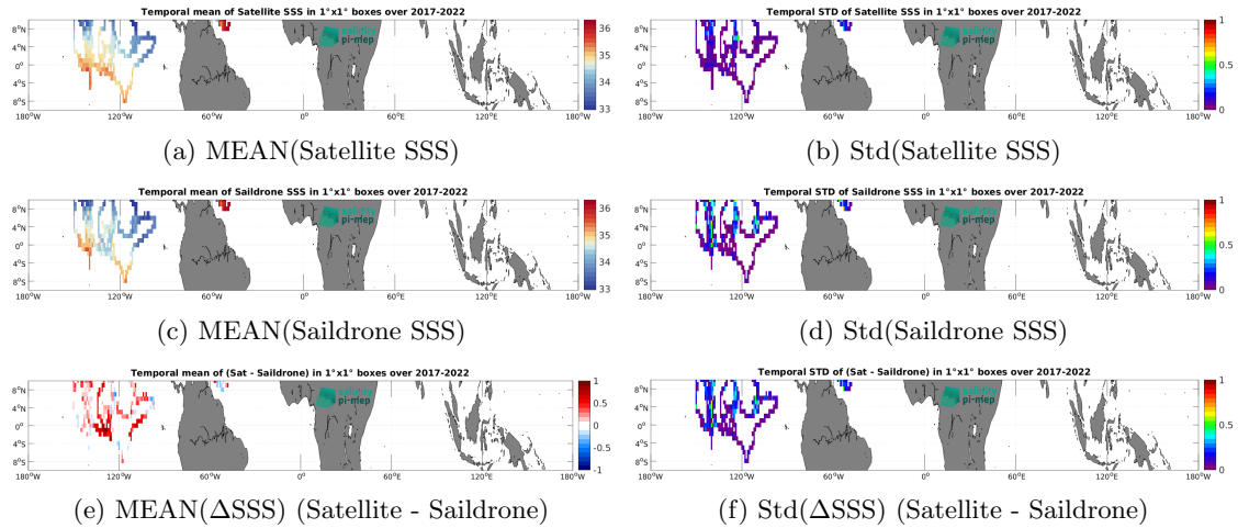
Figure 6: Temporal mean (left) and Std (right) of SSS from SMOS SSS L3 v8 - 18 Days (CATDS-CEC-LOCEAN) (top), Saildrone (middle), and of \Delta SSS (Satellite - Saildrone). Only match-up pairs are used to generate these maps.
