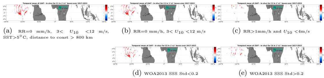
Figure 12: Temporal mean gridded over spatial boxes of size 1^\circ \times 1^\circ of \Delta SSS (SMOS SSS L3 v8 - 18 Days (CATDS-CEC-LOCEAN) - Saildrone) for 5 different subdatasets corresponding to: RR=0 mm/h, 3 < U_{10} < 12 m/s, SST >5^\circ\text{C} , distance to coast > 800 km (a), RR=0 mm/h, 3 < U_{10} < 12 m/s (b), RR >1 mm/h and U_{10} < 4 m/s (c), WOA2013 SSS Std <0.2 (d), WOA2013 SSS Std >0.2 (e).
