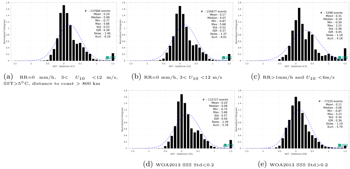
Figure 13: Normalized histogram of \Delta SSS (SMOS SSS L3 v8 - 18 Days (CATDS-CEC-LOCEAN) - Saildrone) for 5 different subdatasets corresponding to: RR=0 mm/h, 3 < U_{10} < 12 m/s, SST >5^\circ\text{C} , distance to coast > 800 km (a), RR=0 mm/h, 3 < U_{10} < 12 m/s (b), RR >1 mm/h and U_{10} < 4 m/s (c), WOA2013 SSS Std <0.2 (d), WOA2013 SSS Std >0.2 (e).
