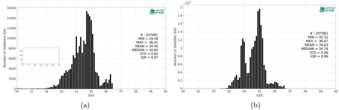
Figure 2: Histograms of SSS from Saildrone (a) and SMOS SSS L3 v8 - 18 Days (CATDS-CEC-LOCEAN) (b) considering all match-up pairs per bins of 0.1 over the Equatorial Ocean 10N-10S Pi-MEP region and for the full satellite product period.
