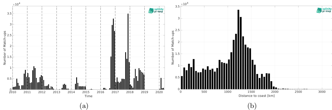
Figure 1: Number of match-ups between Surface drifters and SMOS SSS L3 v8 - 18 Days (CATDS-CEC-LOCEAN) SSS as a function of time (a) and as function of the distance to coast (b) over the Equatorial Ocean 10N-10S Pi-MEP region and for the full satellite product period.
