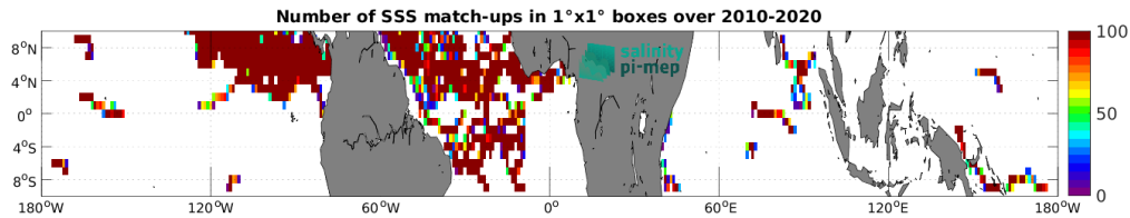
Figure 3: Number of SSS match-ups between Surface drifters SSS and the SMOS SSS L3 v8 - 18 Days (CATDS-CEC-LOCEAN) SSS product for the Equatorial Ocean 10N-10S Pi-MEP region over 1^\circ \times 1^\circ boxes and for the full satellite product period.
