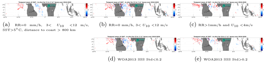
Figure 11: Temporal mean gridded over spatial boxes of size 1^\circ \times 1^\circ of \Delta SSS (SMOS SSS L3 v8 - 18 Days (CATDS-CEC-LOCEAN) - Surface drifters) for 5 different subdatasets corresponding to: RR=0 mm/h, 3 < U_{10} < 12 m/s, SST >5^\circ C, distance to coast > 800 km (a), RR=0 mm/h, 3 < U_{10} < 12 m/s (b), RR >1 mm/h and U_{10} < 4 m/s (c), WOA2013 SSS Std <0.2 (d), WOA2013 SSS Std >0.2 (e).
