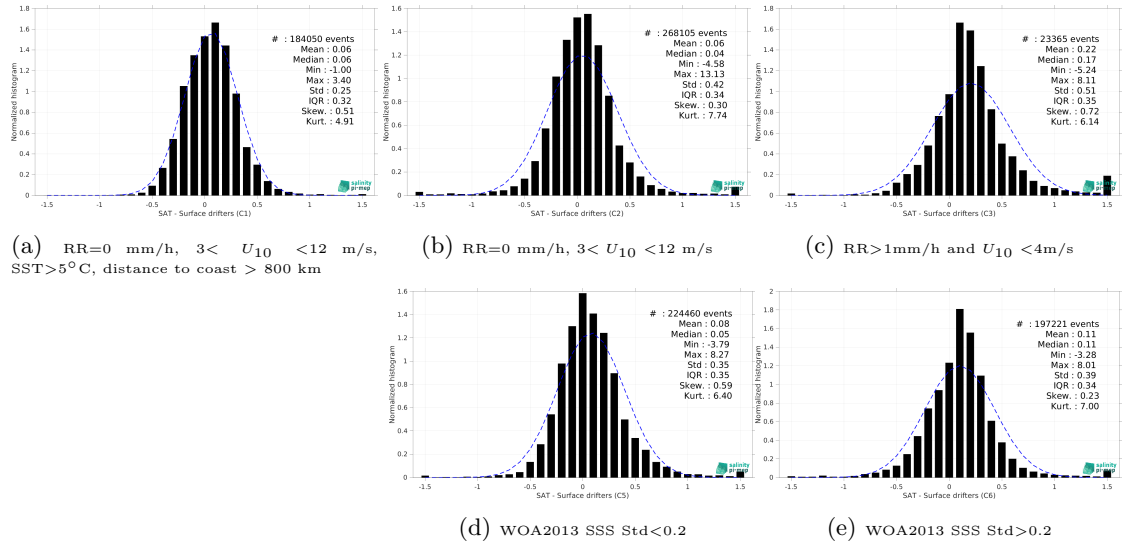
Figure 12: Normalized histogram of \Delta SSS (SMOS SSS L3 v8 - 18 Days (CATDS-CEC-LOCEAN) - Surface drifters) for 5 different subdatasets corresponding to: RR=0 mm/h, 3 < U_{10} < 12 m/s, SST >5^\circ C, distance to coast > 800 km (a), RR=0 mm/h, 3 < U_{10} < 12 m/s (b), RR >1 mm/h and U_{10} < 4 m/s (c), WOA2013 SSS Std <0.2 (d), WOA2013 SSS Std >0.2 (e).
