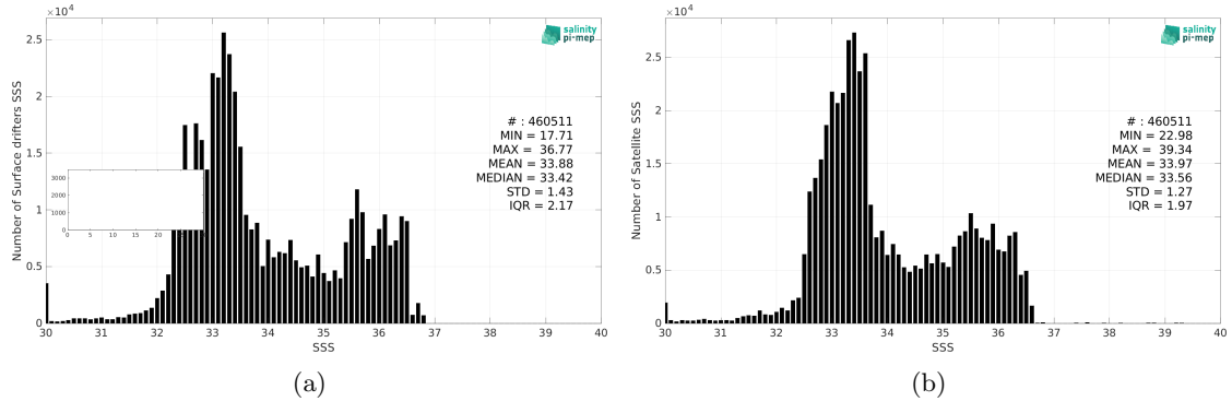
Figure 2: Histograms of SSS from Surface drifters (a) and SMOS SSS L3 v8 - 18 Days (CATDS-CEC-LOCEAN) (b) considering all match-up pairs per bins of 0.1 over the Equatorial Ocean 10N-10S Pi-MEP region and for the full satellite product period.
