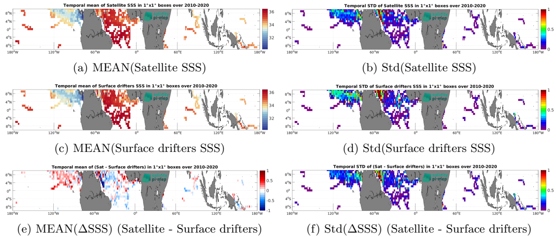
Figure 5: Temporal mean (left) and Std (right) of SSS from SMOS SSS L3 v8 - 18 Days (CATDS-CEC-LOCEAN) (top), Surface drifters (middle), and of \Delta SSS (Satellite - Surface drifters). Only match-up pairs are used to generate these maps.
