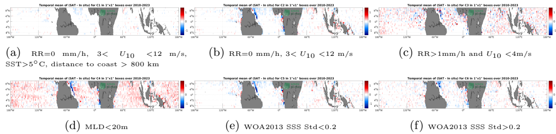
Figure 12: Temporal mean gridded over spatial boxes of size 1^\circ \times 1^\circ of \Delta SSS (SMOS SSS L3 v8 - 18 Days (CATDS-CECOS-LOCEAN) - Argo) for 6 different subdatasets corresponding to:RR=0 mm/h, 3 < U_{10} < 12 m/s, SST >5^\circ C, distance to coast > 800 km (a), RR=0 mm/h, 3 < U_{10} < 12 m/s (b), RR >1 mm/h and U_{10} < 4 m/s (c),MLD <20 m (d),WOA2013 SSS Std <0.2 (e),WOA2013 SSS Std >0.2 (f).
