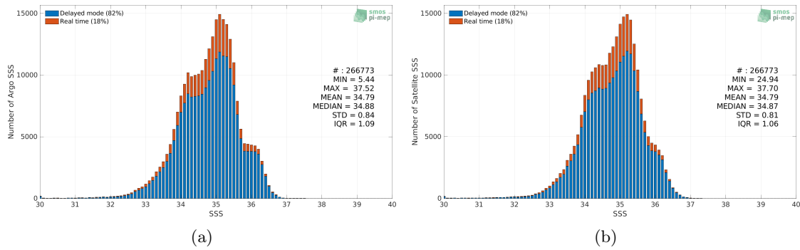
Figure 2: Histograms of SSS from Argo (a) and SMOS SSS L3 v8 - 18 Days (CATDS-CECOS-LOCEAN) (b) considering all match-up pairs per bins of 0.1 over the Equatorial Ocean 10N-10S Pi-MEP region and for the full satellite product period.
