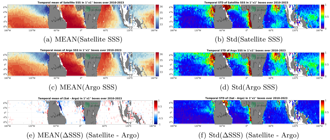
Figure 6: Temporal mean (left) and Std (right) of SSS from SMOS SSS L3 v8 - 18 Days (CATDS-CECOS-LOCEAN) (top), Argo (middle), and of \Delta SSS (Satellite - Argo). Only match-up pairs are used to generate these maps.
