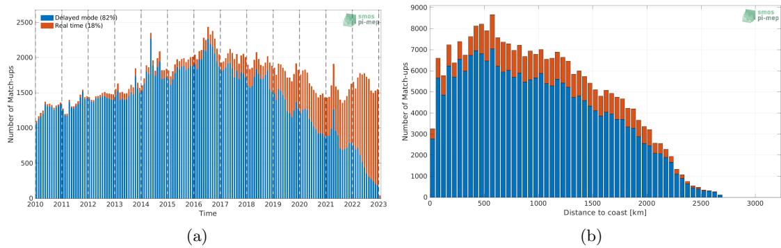
Figure 1: Number of match-ups between Argo and SMOS SSS L3 v8 - 18 Days (CATDS-CECOS-LOCEAN) SSS as a function of time (a) and as function of the distance to coast (b) over the Equatorial Ocean 10N-10S Pi-MEP region and for the full satellite product period.
