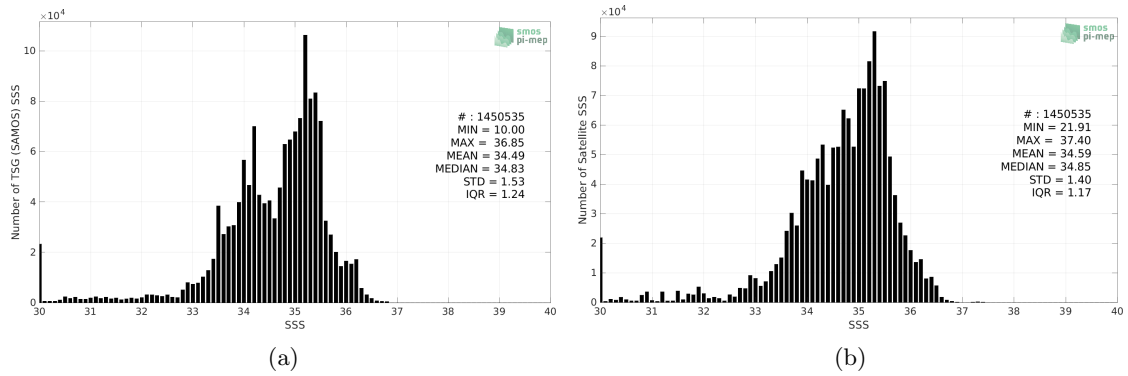
Figure 2: Histograms of SSS from TSG (SAMOS) (a) and SMOS SSS L3 v7 - 9 Days (CATDS-CECOS-LOCEAN) (b) considering all match-up pairs per bins of 0.1 over the Equatorial Ocean 10N-10S Pi-MEP region and for the full satellite product period.
