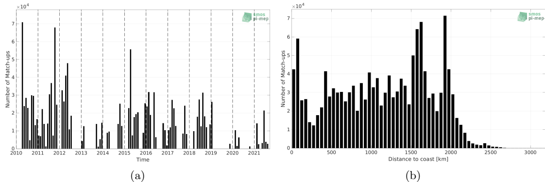
Figure 1: Number of match-ups between TSG (SAMOS) and SMOS SSS L3 v7 - 9 Days (CATDS-CECOS-LOCEAN) SSS as a function of time (a) and as function of the distance to coast (b) over the Equatorial Ocean 10N-10S Pi-MEP region and for the full satellite product period.
