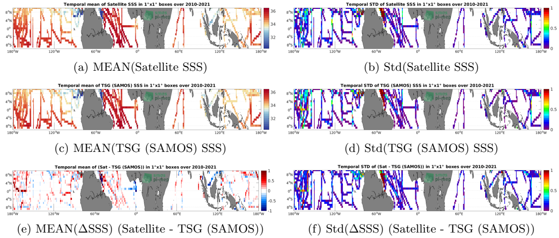
Figure 6: Temporal mean (left) and Std (right) of SSS from SMOS SSS L3 v7 - 9 Days (CATDS-CECOS-LOCEAN) (top), TSG (SAMOS) in situ dataset (middle), and of \Delta SSS (Satellite - TSG (SAMOS)). Only match-up pairs are used to generate these maps.
