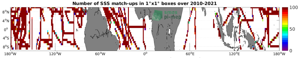
Figure 4: Number of SSS match-ups between TSG (SAMOS) SSS and the SMOS SSS L3 v7 - 9 Days (CATDS-CECOS-LOCEAN) SSS product for the Equatorial Ocean 10N-10S Pi-MEP region over 1^\circ \times 1^\circ boxes and for the full satellite product period.
