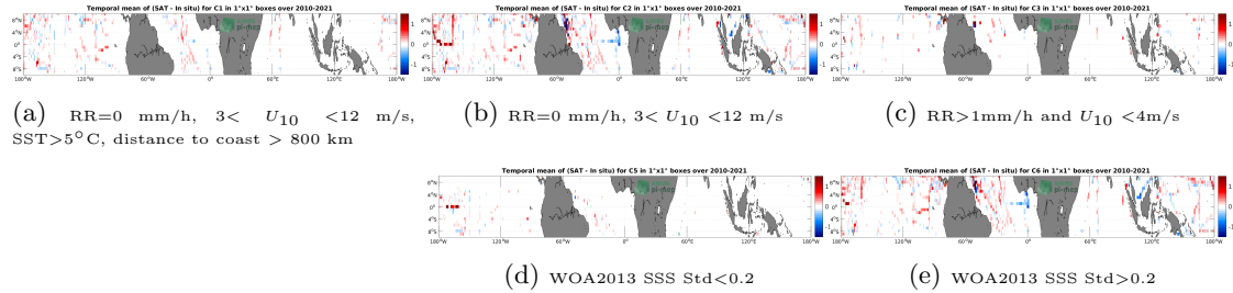
Figure 12: Temporal mean gridded over spatial boxes of size 1^{\circ}\times 1^{\circ} of \Delta\text{SSS} (SMOS SSS L3 v7 - 9 Days (CATDS-CECOS-LOCEAN) - TSG (SAMOS)) for 5 different subdatasets corresponding to:RR=0 mm/h, 3 < U_{10} < 12 m/s, SST >5^{\circ}\text{C} , distance to coast > 800 km (a), RR=0 mm/h, 3 < U_{10} < 12 m/s (b), RR >1 mm/h and U_{10} < 4 m/s (c), WOA2013 SSS Std <0.2 (d), WOA2013 SSS Std >0.2 (e).
