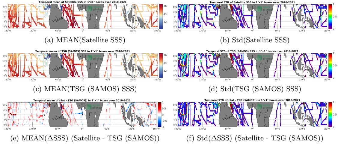
Figure 6: Temporal mean (left) and Std (right) of SSS from SMOS SSS L3 v7 - 9 Days (CATDS-CECOS-LOCEAN) (top), TSG (SAMOS) (middle), and of \Delta SSS (Satellite - TSG (SAMOS)). Only match-up pairs are used to generate these maps.
