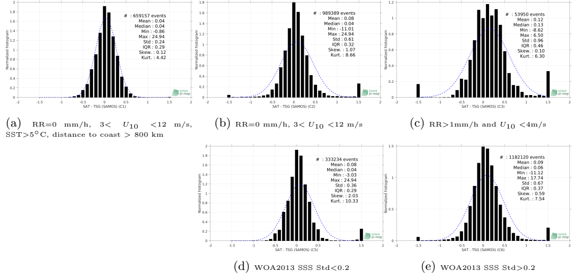
Figure 13: Normalized histogram of \Delta\text{SSS} (SMOS SSS L3 v7 - 9 Days (CATDS-CECOS-LOCEAN) - TSG (SAMOS)) for 5 different subdatasets corresponding to: RR=0 mm/h, 3 < U_{10} < 12 m/s, SST>5°C, distance to coast > 800 km (a), RR=0 mm/h, 3 < U_{10} < 12 m/s (b), RR>1mm/h and U_{10} < 4 m/s (c), WOA2013 SSS Std<0.2 (d), WOA2013 SSS Std>0.2 (e).
