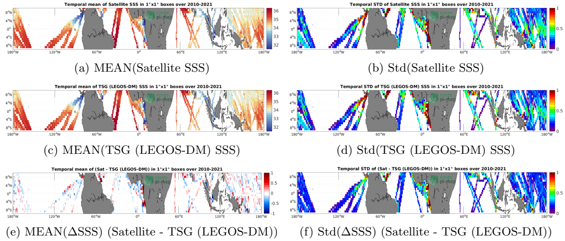
Figure 6: Temporal mean (left) and Std (right) of SSS from SMOS SSS L3 v7 - 9 Days (CATDS-CECOS-LOCEAN) (top), TSG (LEGOS-DM) ( in situ ) dataset (middle), and of \Delta SSS (Satellite - TSG (LEGOS-DM)). Only match-up pairs are used to generate these maps.
