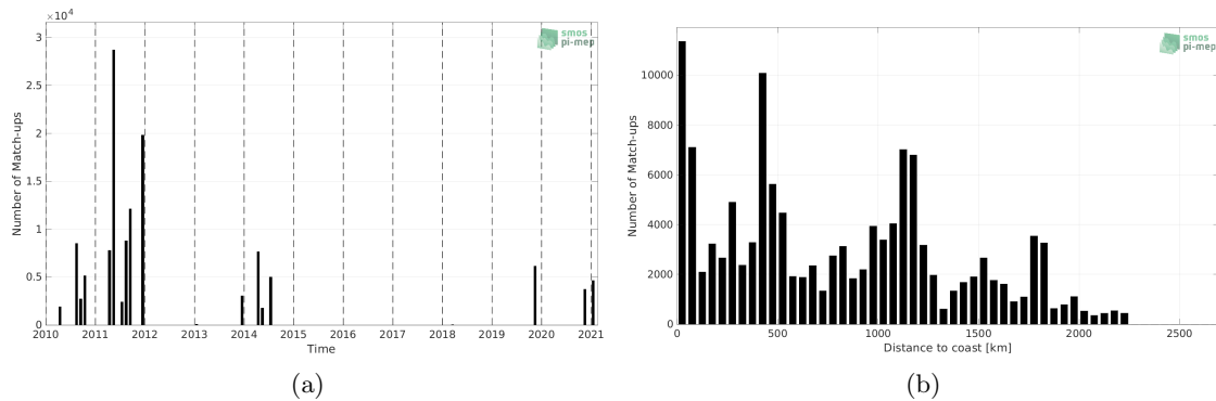
Figure 1: Number of match-ups between TSG (GOSUD-Sailing-ship) and SMOS SSS L3 v7 - 9 Days (CATDS-CECOS-LOCEAN) SSS as a function of time (a) and as function of the distance to coast (b) over the Equatorial Ocean 10N-10S Pi-MEP region and for the full satellite product period.
