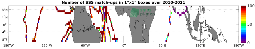
Figure 4: Number of SSS match-ups between TSG (GOSUD-Sailing-ship) SSS and the SMOS SSS L3 v7 - 9 Days (CATDS-CECOS-LOCEAN) SSS product for the Equatorial Ocean 10N-10S Pi-MEP region over 1^\circ \times 1^\circ boxes and for the full satellite product period.
