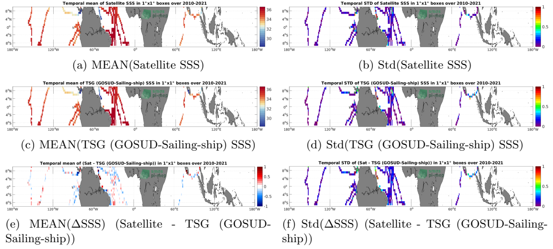
Figure 6: Temporal mean (left) and Std (right) of SSS from SMOS SSS L3 v7 - 9 Days (CATDS-CECOS-LOCEAN) (top), TSG (GOSUD-Sailing-ship) (middle), and of \Delta SSS (Satellite - TSG (GOSUD-Sailing-ship)). Only match-up pairs are used to generate these maps.
