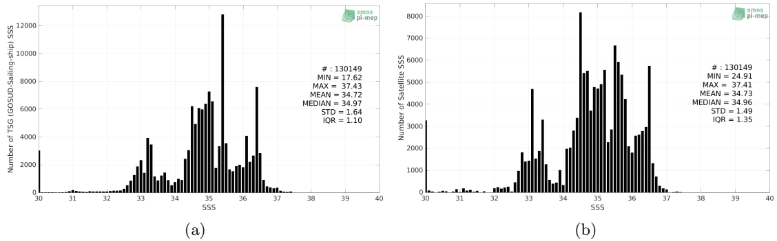
Figure 2: Histograms of SSS from TSG (GOSUD-Sailing-ship) (a) and SMOS SSS L3 v7 - 9 Days (CATDS-CECOS-LOCEAN) (b) considering all match-up pairs per bins of 0.1 over the Equatorial Ocean 10N-10S Pi-MEP region and for the full satellite product period.
