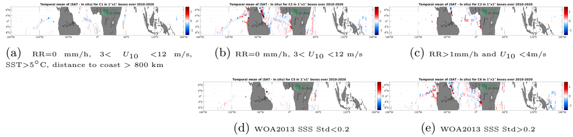
Figure 12: Temporal mean gridded over spatial boxes of size 1^{\circ}\times 1^{\circ} of \Delta SSS (SMOS SSS L3 v7 - 9 Days (CATDS-CECOS-LOCEAN) - TSG (GOSUD-Research-vessel)) for 5 different subdatasets corresponding to:RR=0 mm/h, 3 < U_{10} < 12 m/s, SST >5^{\circ}\text{C} , distance to coast > 800 km (a), RR=0 mm/h, 3 < U_{10} < 12 m/s (b), RR >1 mm/h and U_{10} < 4 m/s (c), WOA2013 SSS Std <0.2 (d), WOA2013 SSS Std >0.2 (e).
