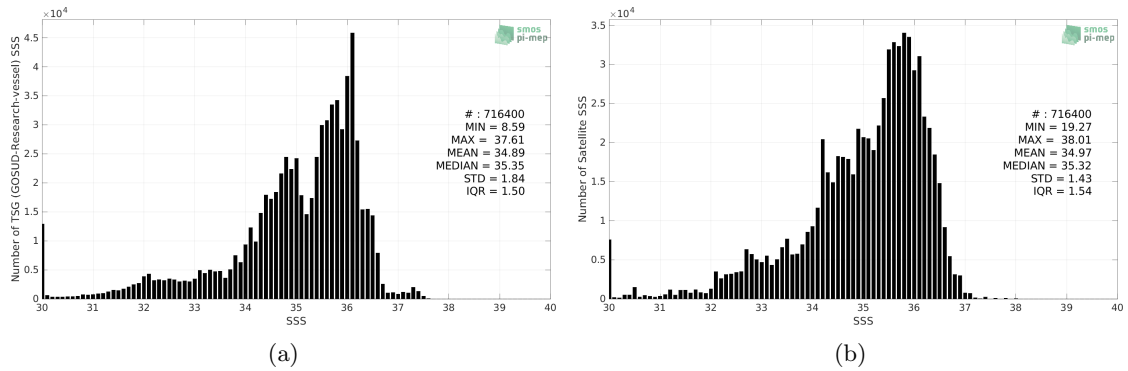
Figure 2: Histograms of SSS from TSG (GOSUD-Research-vessel) (a) and SMOS SSS L3 v7 - 9 Days (CATDS-CECOS-LOCEAN) (b) considering all match-up pairs per bins of 0.1 over the Equatorial Ocean 10N-10S Pi-MEP region and for the full satellite product period.
