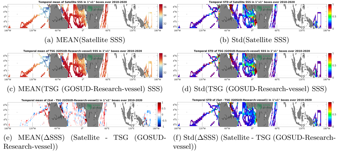
Figure 6: Temporal mean (left) and Std (right) of SSS from SMOS SSS L3 v7 - 9 Days (CATDS-CECOS-LOCEAN) (top), TSG (GOSUD-Research-vessel) (middle), and of \Delta SSS (Satellite - TSG (GOSUD-Research-vessel)). Only match-up pairs are used to generate these maps.
