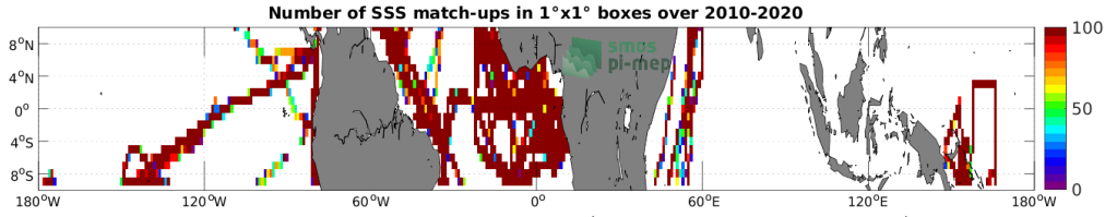
Figure 4: Number of SSS match-ups between TSG (GOSUD-Research-vessel) SSS and the SMOS SSS L3 v7 - 9 Days (CATDS-CECOS-LOCEAN) SSS product for the Equatorial Ocean 10N-10S Pi-MEP region over 1^\circ \times 1^\circ boxes and for the full satellite product period.
