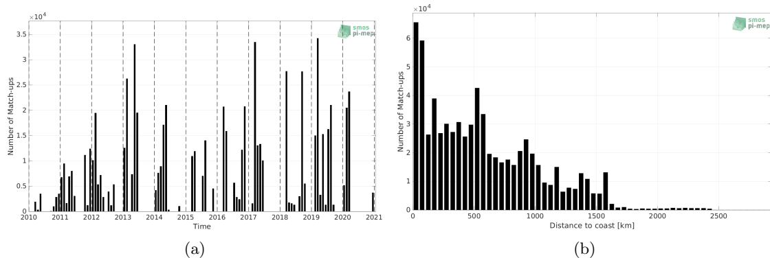
Figure 1: Number of match-ups between TSG (GOSUD-Research-vessel) and SMOS SSS L3 v7 - 9 Days (CATDS-CECOS-LOCEAN) SSS as a function of time (a) and as function of the distance to coast (b) over the Equatorial Ocean 10N-10S Pi-MEP region and for the full satellite product period.
