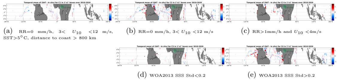
Figure 12: Temporal mean gridded over spatial boxes of size 1^\circ \times 1^\circ of \Delta SSS (SMOS SSS L3 v7 - 9 Days (CATDS-CECOS-LOCEAN) - TSG (GOSUD-Research-vessel)) for 5 different subdatasets corresponding to:RR=0 mm/h, 3 < U_{10} < 12 m/s, SST > 5^\circ\text{C} , distance to coast > 800 km (a), RR=0 mm/h, 3 < U_{10} < 12 m/s (b), RR > 1 mm/h and U_{10} < 4 m/s (c), WOA2013 SSS Std < 0.2 (d), WOA2013 SSS Std > 0.2 (e).
