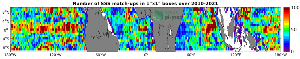
Figure 4: Number of SSS match-ups between Argo SSS and the SMOS SSS L3 v7 - 9 Days (CATDS-CECOS-LOCEAN) SSS product for the Equatorial Ocean 10N-10S Pi-MEP region over 1^\circ \times 1^\circ boxes and for the full satellite product period.
