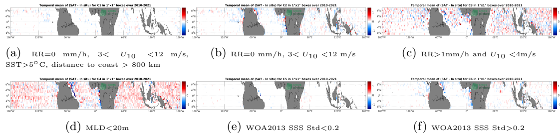
Figure 12: Temporal mean gridded over spatial boxes of size 1^\circ \times 1^\circ of \Delta SSS (SMOS SSS L3 v7 - 9 Days (CATDS-CECOS-LOCEAN) - Argo) for 6 different subdatasets corresponding to:RR=0 mm/h, 3 < U_{10} < 12 m/s, SST >5^\circ C, distance to coast > 800 km (a), RR=0 mm/h, 3 < U_{10} < 12 m/s (b), RR >1 mm/h and U_{10} < 4 m/s (c),MLD <20 m (d),WOA2013 SSS Std <0.2 (e),WOA2013 SSS Std >0.2 (f).
