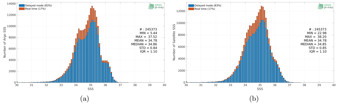
Figure 2: Histograms of SSS from Argo (a) and SMOS SSS L3 v7 - 9 Days (CATDS-CECOS-LOCEAN) (b) considering all match-up pairs per bins of 0.1 over the Equatorial Ocean 10N-10S Pi-MEP region and for the full satellite product period.
