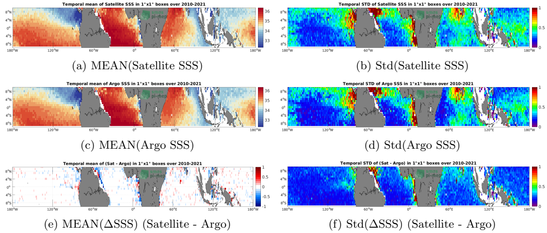
Figure 6: Temporal mean (left) and Std (right) of SSS from SMOS SSS L3 v7 - 9 Days (CATDS-CECOS-LOCEAN) (top), Argo (middle), and of \Delta SSS (Satellite - Argo). Only match-up pairs are used to generate these maps.
