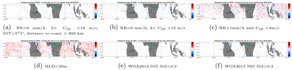
Figure 12: Temporal mean gridded over spatial boxes of size 1^\circ \times 1^\circ of \Delta SSS (SMOS SSS L3 v7 - 9 Days (CATDS-CECOS-LOCEAN) - Argo) for 6 different subdatasets corresponding to:RR=0 mm/h, 3 < U_{10} < 12 m/s, SST >5^\circ C, distance to coast > 800 km (a), RR=0 mm/h, 3 < U_{10} < 12 m/s (b), RR >1 mm/h and U_{10} < 4 m/s (c),MLD <20 m (d),WOA2013 SSS Std <0.2 (e),WOA2013 SSS Std >0.2 (f).
