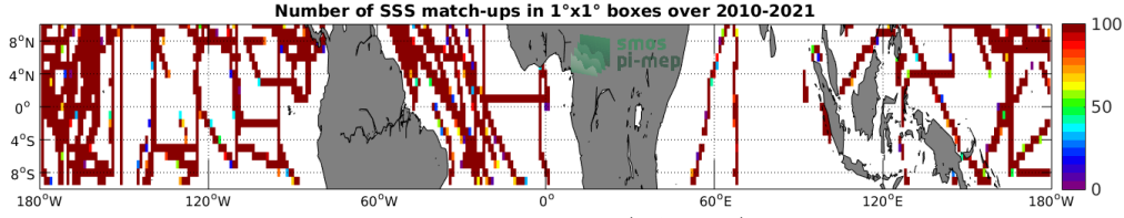
Figure 4: Number of SSS match-ups between TSG (SAMOS) SSS and the SMOS SSS L3 v7 - 18 Days (CATDS-CECOS-LOCEAN) SSS product for the Equatorial Ocean 10N-10S Pi-MEP region over 1^\circ \times 1^\circ boxes and for the full satellite product period.
