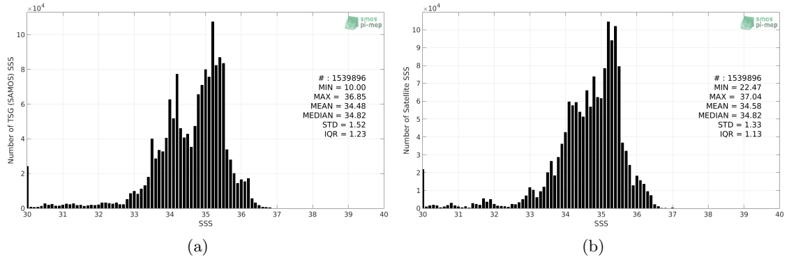
Figure 2: Histograms of SSS from TSG (SAMOS) (a) and SMOS SSS L3 v7 - 18 Days (CATDS-CECOS-LOCEAN) (b) considering all match-up pairs per bins of 0.1 over the Equatorial Ocean 10N-10S Pi-MEP region and for the full satellite product period.
