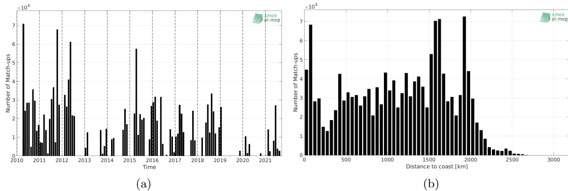
Figure 1: Number of match-ups between TSG (SAMOS) and SMOS SSS L3 v7 - 18 Days (CATDS-CECOS-LOCEAN) SSS as a function of time (a) and as function of the distance to coast (b) over the Equatorial Ocean 10N-10S Pi-MEP region and for the full satellite product period.
