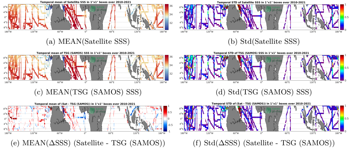
Figure 6: Temporal mean (left) and Std (right) of SSS from SMOS SSS L3 v7 - 18 Days (CATDS-CECOS-LOCEAN) (top), TSG (SAMOS) (middle), and of \Delta SSS (Satellite - TSG (SAMOS)). Only match-up pairs are used to generate these maps.
