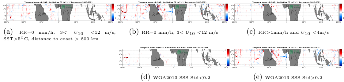
Figure 12: Temporal mean gridded over spatial boxes of size 1^{\circ}\times 1^{\circ} of \Delta\text{SSS} (SMOS SSS L3 v7 - 18 Days (CATDS-CECOS-LOCEAN) - TSG (SAMOS)) for 5 different subdatasets corresponding to:RR=0 mm/h, 3 < U_{10} < 12 m/s, SST >5^{\circ}\text{C} , distance to coast > 800 km (a), RR=0 mm/h, 3 < U_{10} < 12 m/s (b), RR >1 mm/h and U_{10} < 4 m/s (c), WOA2013 SSS Std <0.2 (d), WOA2013 SSS Std >0.2 (e).
