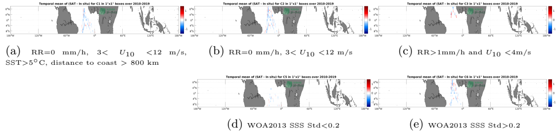
Figure 12: Temporal mean gridded over spatial boxes of size 1^{\circ}\times 1^{\circ} of \Delta\text{SSS} (SMOS SSS L3 v7 - 18 Days (CATDS-CECOS-LOCEAN) - TSG (Polarstern)) for 5 different subdatasets corresponding to:RR=0 mm/h, 3 < U_{10} < 12 m/s, SST >5^{\circ}\text{C} , distance to coast > 800 km (a), RR=0 mm/h, 3 < U_{10} < 12 m/s (b), RR >1 mm/h and U_{10} < 4 m/s (c), WOA2013 SSS Std <0.2 (d), WOA2013 SSS Std >0.2 (e).
