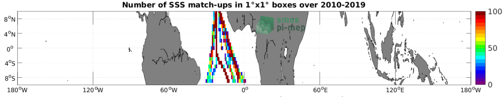
Figure 4: Number of SSS match-ups between TSG (Polarstern) SSS and the SMOS SSS L3 v7 - 18 Days (CATDS-CECOS-LOCEAN) SSS product for the Equatorial Ocean 10N-10S Pi-MEP region over 1^\circ \times 1^\circ boxes and for the full satellite product period.
