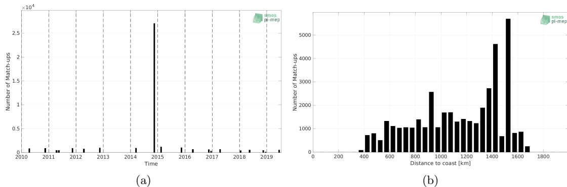
Figure 1: Number of match-ups between TSG (Polarstern) and SMOS SSS L3 v7 - 18 Days (CATDS-CECOS-LOCEAN) SSS as a function of time (a) and as function of the distance to coast (b) over the Equatorial Ocean 10N-10S Pi-MEP region and for the full satellite product period.
