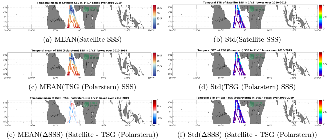
Figure 6: Temporal mean (left) and Std (right) of SSS from SMOS SSS L3 v7 - 18 Days (CATDS-CECOS-LOCEAN) (top), TSG (Polarstern) (middle), and of \Delta SSS (Satellite - TSG (Polarstern)). Only match-up pairs are used to generate these maps.
