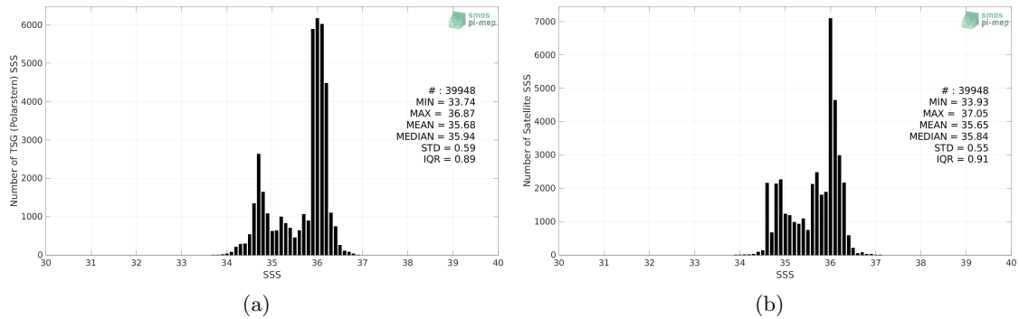
Figure 2: Histograms of SSS from TSG (Polarstern) (a) and SMOS SSS L3 v7 - 18 Days (CATDS-CECOS-LOCEAN) (b) considering all match-up pairs per bins of 0.1 over the Equatorial Ocean 10N-10S Pi-MEP region and for the full satellite product period.
