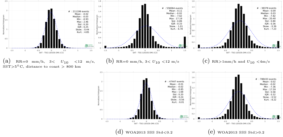
Figure 13: Normalized histogram of \Delta\text{SSS} (SMOS SSS L3 v7 - 18 Days (CATDS-CECOS-LOCEAN) - TSG (LEGOS-DM)) for 5 different subdatasets corresponding to: RR=0 mm/h, 3 < U_{10} < 12 m/s, SST>5°C, distance to coast > 800 km (a), RR=0 mm/h, 3 < U_{10} < 12 m/s (b), RR>1mm/h and U_{10} < 4 m/s (c), WOA2013 SSS Std<0.2 (d), WOA2013 SSS Std>0.2 (e).
