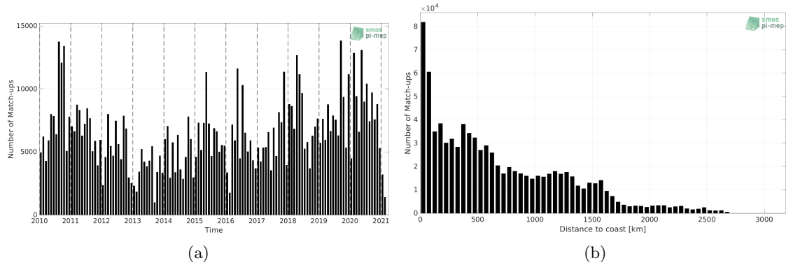
Figure 1: Number of match-ups between TSG (LEGOS-DM) and SMOS SSS L3 v7 - 18 Days (CATDS-CECOS-LOCEAN) SSS as a function of time (a) and as function of the distance to coast (b) over the Equatorial Ocean 10N-10S Pi-MEP region and for the full satellite product period.
