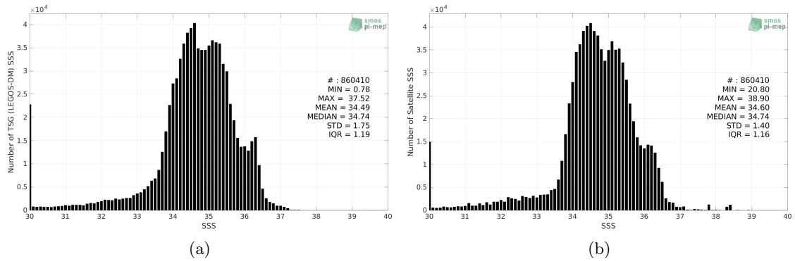
Figure 2: Histograms of SSS from TSG (LEGOS-DM) (a) and SMOS SSS L3 v7 - 18 Days (CATDS-CECOS-LOCEAN) (b) considering all match-up pairs per bins of 0.1 over the Equatorial Ocean 10N-10S Pi-MEP region and for the full satellite product period.
