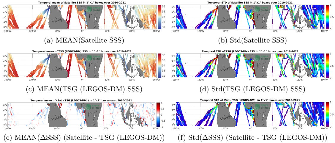
Figure 6: Temporal mean (left) and Std (right) of SSS from SMOS SSS L3 v7 - 18 Days (CATDS-CECOS-LOCEAN) (top), TSG (LEGOS-DM) (middle), and of \Delta SSS (Satellite - TSG (LEGOS-DM)). Only match-up pairs are used to generate these maps.
