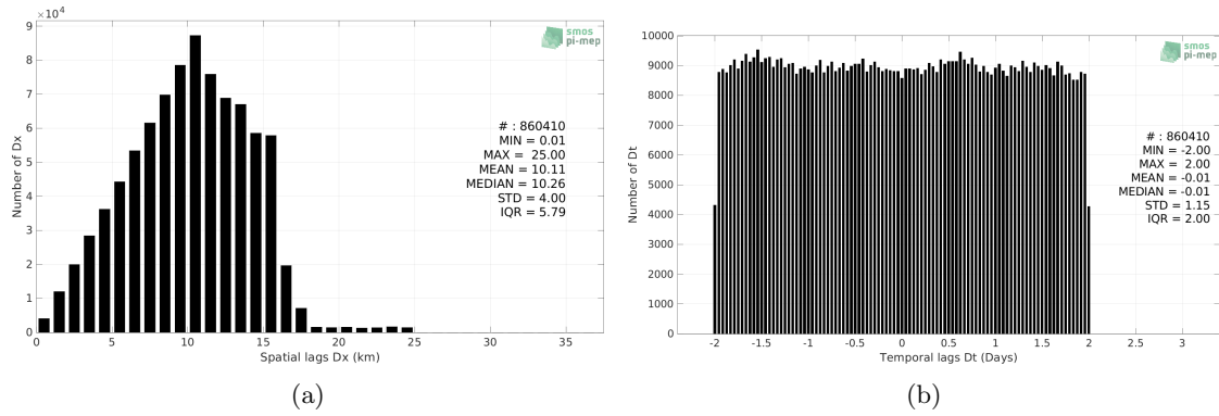
Figure 5: Histograms of the spatial (a) and temporal (b) lags between the location/time of the TSG (LEGOS-DM) measurement and the date of the corresponding SMOS SSS L3 v7 - 18 Days (CATDS-CECOS-LOCEAN) SSS pixel.
