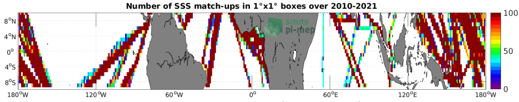
Figure 4: Number of SSS match-ups between TSG (LEGOS-DM) SSS and the SMOS SSS L3 v7 - 18 Days (CATDS-CECOS-LOCEAN) SSS product for the Equatorial Ocean 10N-10S Pi-MEP region over 1^\circ \times 1^\circ boxes and for the full satellite product period.
