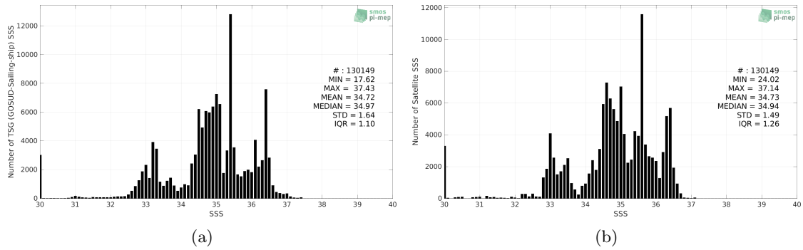
Figure 2: Histograms of SSS from TSG (GOSUD-Sailing-ship) (a) and SMOS SSS L3 v7 - 18 Days (CATDS-CECOS-LOCEAN) (b) considering all match-up pairs per bins of 0.1 over the Equatorial Ocean 10N-10S Pi-MEP region and for the full satellite product period.
