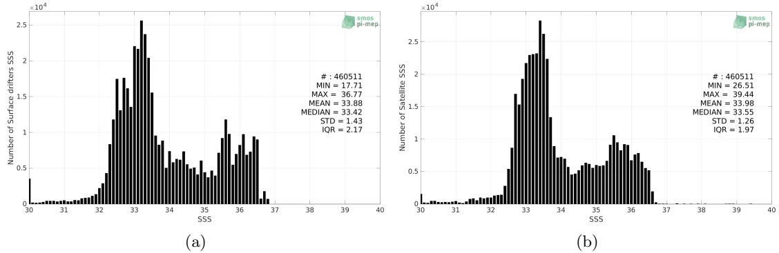
Figure 2: Histograms of SSS from Surface drifters (a) and SMOS SSS L3 v7 - 18 Days (CATDS-CECOS-LOCEAN) (b) considering all match-up pairs per bins of 0.1 over the Equatorial Ocean 10N-10S Pi-MEP region and for the full satellite product period.
