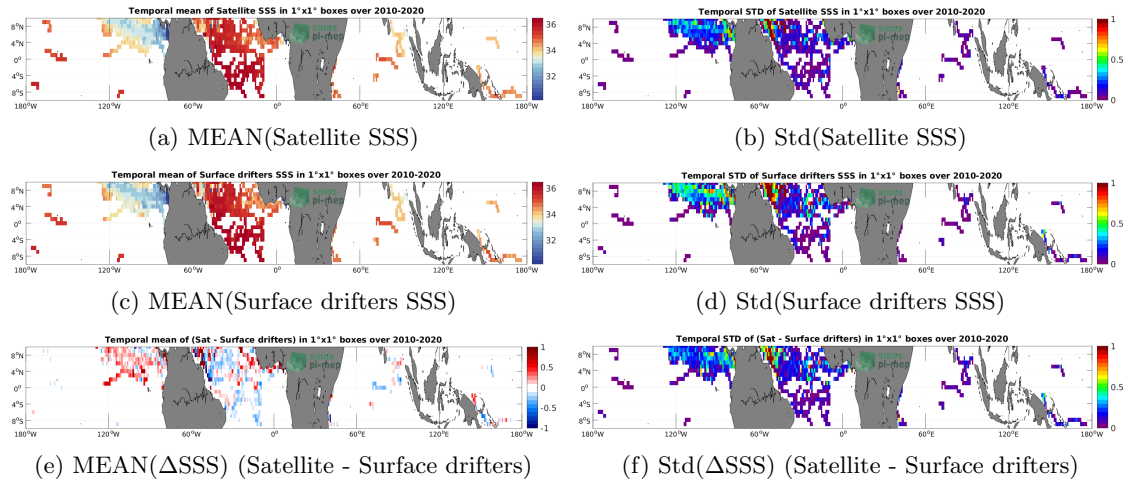
Figure 5: Temporal mean (left) and Std (right) of SSS from SMOS SSS L3 v7 - 18 Days (CATDS-CECOS-LOCEAN) (top), Surface drifters (middle), and of \Delta SSS (Satellite - Surface drifters). Only match-up pairs are used to generate these maps.
