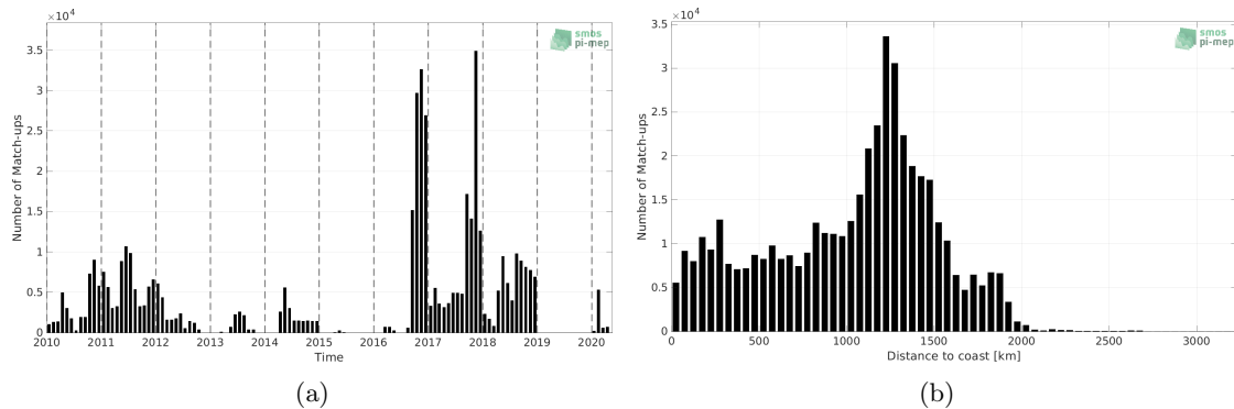
Figure 1: Number of match-ups between Surface drifters and SMOS SSS L3 v7 - 18 Days (CATDS-CECOS-LOCEAN) SSS as a function of time (a) and as function of the distance to coast (b) over the Equatorial Ocean 10N-10S Pi-MEP region and for the full satellite product period.
