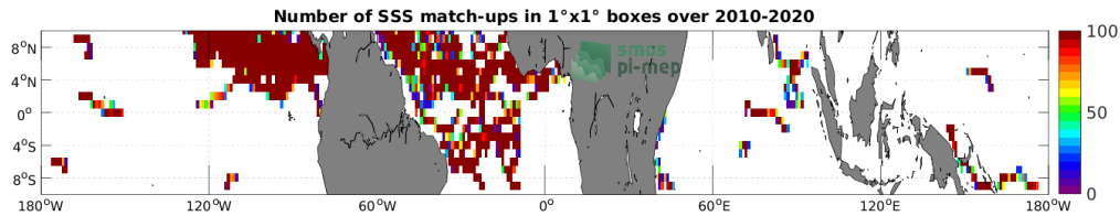
Figure 3: Number of SSS match-ups between Surface drifters SSS and the SMOS SSS L3 v7 - 18 Days (CATDS-CECOS-LOCEAN) SSS product for the Equatorial Ocean 10N-10S Pi-MEP region over 1^\circ \times 1^\circ boxes and for the full satellite product period.
