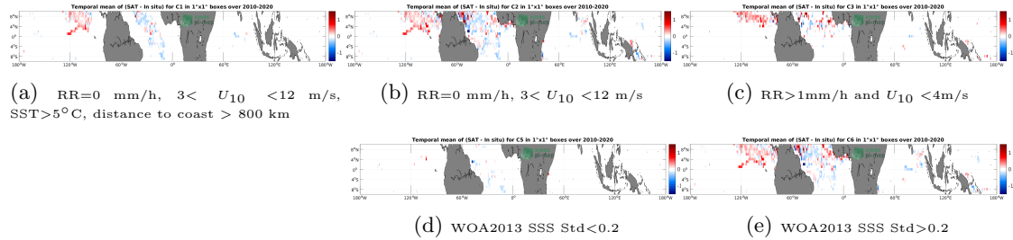
Figure 11: Temporal mean gridded over spatial boxes of size 1^{\circ}\times 1^{\circ} of \Delta\text{SSS} (SMOS SSS L3 v7 - 18 Days (CATDS-CECOS-LOCEAN) - Surface drifters) for 5 different subdatasets corresponding to:RR=0 mm/h, 3 < U_{10} < 12 m/s, SST >5^{\circ}\text{C} , distance to coast > 800 km (a), RR=0 mm/h, 3 < U_{10} < 12 m/s (b), RR >1 mm/h and U_{10} < 4 m/s (c), WOA2013 SSS Std <0.2 (d), WOA2013 SSS Std >0.2 (e).
