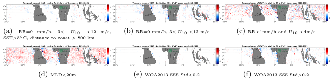
Figure 12: Temporal mean gridded over spatial boxes of size 1^\circ \times 1^\circ of \Delta SSS (SMOS SSS L3 v7 - 18 Days (CATDS-CECOS-LOCEAN) - Argo) for 6 different subdatasets corresponding to:RR=0 mm/h, 3 < U_{10} < 12 m/s, SST >5^\circ C, distance to coast > 800 km (a), RR=0 mm/h, 3 < U_{10} < 12 m/s (b), RR >1 mm/h and U_{10} < 4 m/s (c),MLD <20 m (d),WOA2013 SSS Std <0.2 (e),WOA2013 SSS Std >0.2 (f).
