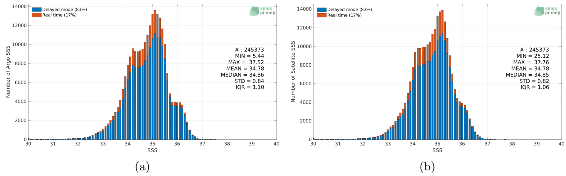
Figure 2: Histograms of SSS from Argo (a) and SMOS SSS L3 v7 - 18 Days (CATDS-CECOS-LOCEAN) (b) considering all match-up pairs per bins of 0.1 over the Equatorial Ocean 10N-10S Pi-MEP region and for the full satellite product period.
