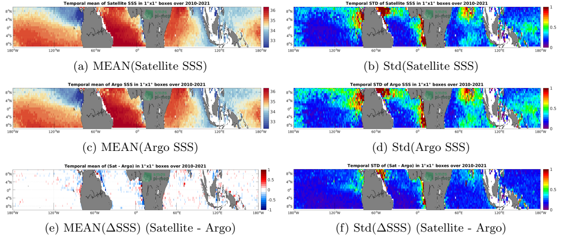
Figure 6: Temporal mean (left) and Std (right) of SSS from SMOS SSS L3 v7 - 18 Days (CATDS-CECOS-LOCEAN) (top), Argo (middle), and of \Delta SSS (Satellite - Argo). Only match-up pairs are used to generate these maps.
