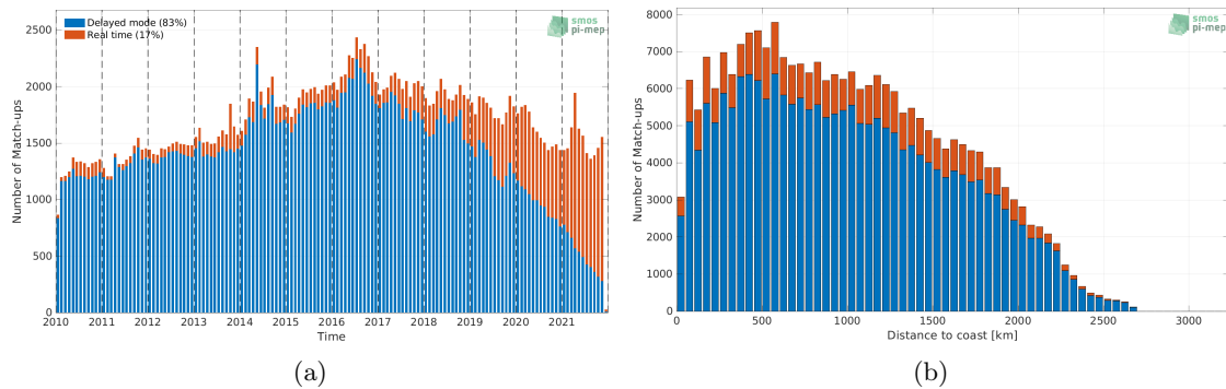
Figure 1: Number of match-ups between Argo and SMOS SSS L3 v7 - 18 Days (CATDS-CECOS-LOCEAN) SSS as a function of time (a) and as function of the distance to coast (b) over the Equatorial Ocean 10N-10S Pi-MEP region and for the full satellite product period.
