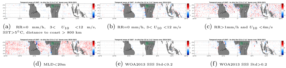
Figure 12: Temporal mean gridded over spatial boxes of size 1^\circ \times 1^\circ of \Delta SSS (SMOS SSS L3 v7 - 18 Days (CATDS-CECOS-LOCEAN) - Argo) for 6 different subdatasets corresponding to:RR=0 mm/h, 3 < U_{10} < 12 m/s, SST > 5^\circ\text{C} , distance to coast > 800 km (a), RR=0 mm/h, 3 < U_{10} < 12 m/s (b), RR > 1 mm/h and U_{10} < 4 m/s (c),MLD < 20 m (d),WOA2013 SSS Std < 0.2 (e),WOA2013 SSS Std > 0.2 (f).
