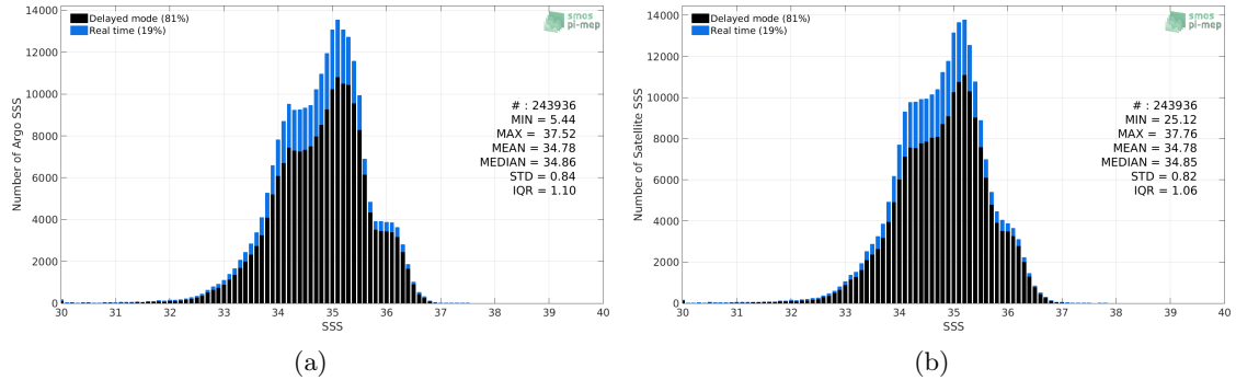
Figure 2: Histograms of SSS from Argo (a) and SMOS SSS L3 v7 - 18 Days (CATDS-CECOS-LOCEAN) (b) considering all match-up pairs per bins of 0.1 over the Equatorial Ocean 10N-10S Pi-MEP region and for the full satellite product period.
