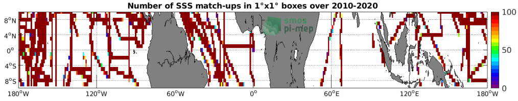
Figure 4: Number of SSS match-ups between TSG (SAMOS) SSS and the SMOS SSS L3 v5 - 9 Days (CATDS-CECOS-LOCEAN) SSS product for the Equatorial Ocean 10N-10S Pi-MEP region over 1^\circ \times 1^\circ boxes and for the full satellite product period.
