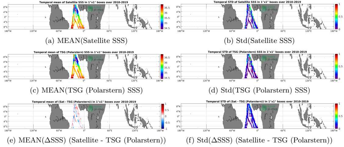
Figure 6: Temporal mean (left) and Std (right) of SSS from SMOS SSS L3 v5 - 9 Days (CATDS-CECOS-LOCEAN) (top), TSG (Polarstern) (middle), and of \Delta SSS (Satellite - TSG (Polarstern)). Only match-up pairs are used to generate these maps.
