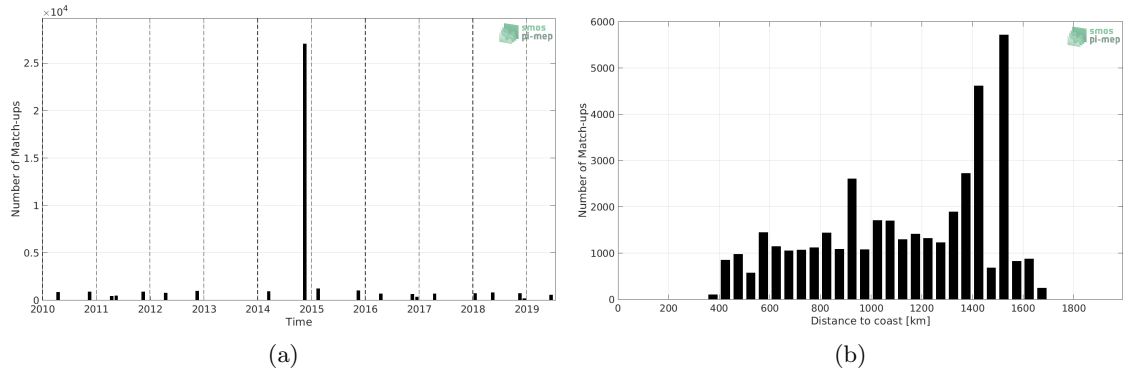
Figure 1: Number of match-ups between TSG (Polarstern) and SMOS SSS L3 v5 - 9 Days (CATDS-CECOS-LOCEAN) SSS as a function of time (a) and as function of the distance to coast (b) over the Equatorial Ocean 10N-10S Pi-MEP region and for the full satellite product period.
