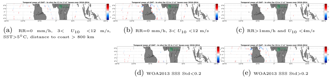
Figure 12: Temporal mean gridded over spatial boxes of size 1^\circ \times 1^\circ of \Delta SSS (SMOS SSS L3 v5 - 9 Days (CATDS-CECOS-LOCEAN) - TSG (GOSUD-Sailing-ship)) for 5 different subdatasets corresponding to: RR=0 mm/h, 3 < U_{10} < 12 m/s, SST > 5^\circ\text{C} , distance to coast > 800 km (a), RR=0 mm/h, 3 < U_{10} < 12 m/s (b), RR > 1 mm/h and U_{10} < 4 m/s (c), WOA2013 SSS Std < 0.2 (d), WOA2013 SSS Std > 0.2 (e).
