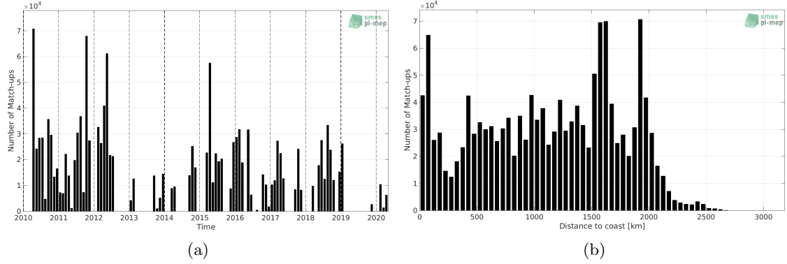
Figure 1: Number of match-ups between TSG (SAMOS) and SMOS SSS L3 v5 - 18 Days (CATDS-CECOS-LOCEAN) SSS as a function of time (a) and as function of the distance to coast (b) over the Equatorial Ocean 10N-10S Pi-MEP region and for the full satellite product period.
