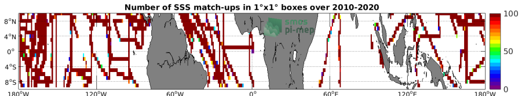
Figure 4: Number of SSS match-ups between TSG (SAMOS) SSS and the SMOS SSS L3 v5 - 18 Days (CATDS-CECOS-LOCEAN) SSS product for the Equatorial Ocean 10N-10S Pi-MEP region over 1^\circ \times 1^\circ boxes and for the full satellite product period.
