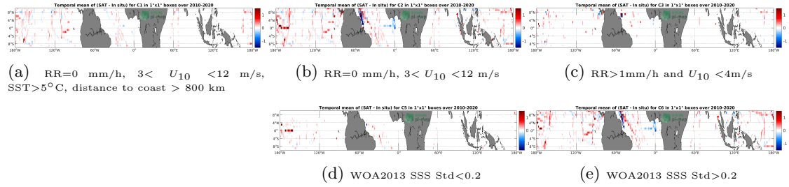
Figure 12: Temporal mean gridded over spatial boxes of size 1^{\circ}\times 1^{\circ} of \Delta\text{SSS} (SMOS SSS L3 v5 - 18 Days (CATDS-CECOS-LOCEAN) - TSG (SAMOS)) for 5 different subdatasets corresponding to:RR=0 mm/h, 3 < U_{10} < 12 m/s, SST >5^{\circ}\text{C} , distance to coast > 800 km (a), RR=0 mm/h, 3 < U_{10} < 12 m/s (b), RR >1 mm/h and U_{10} < 4 m/s (c), WOA2013 SSS Std <0.2 (d), WOA2013 SSS Std >0.2 (e).
