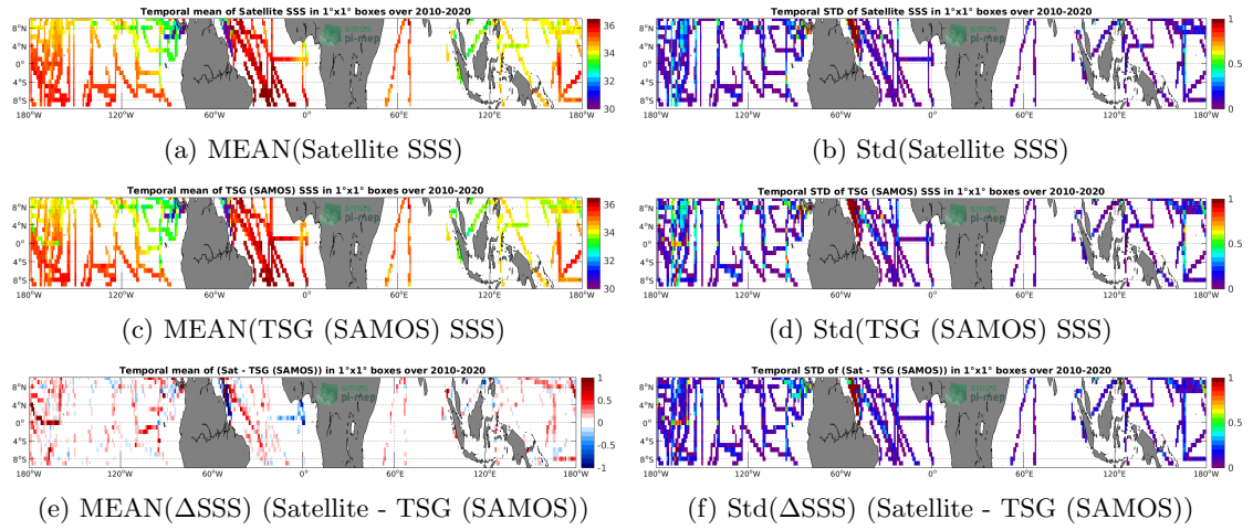
Figure 6: Temporal mean (left) and Std (right) of SSS from SMOS SSS L3 v5 - 18 Days (CATDS-CECOS-LOCEAN) (top), TSG (SAMOS) (middle), and of \Delta SSS (Satellite - TSG (SAMOS)). Only match-up pairs are used to generate these maps.
