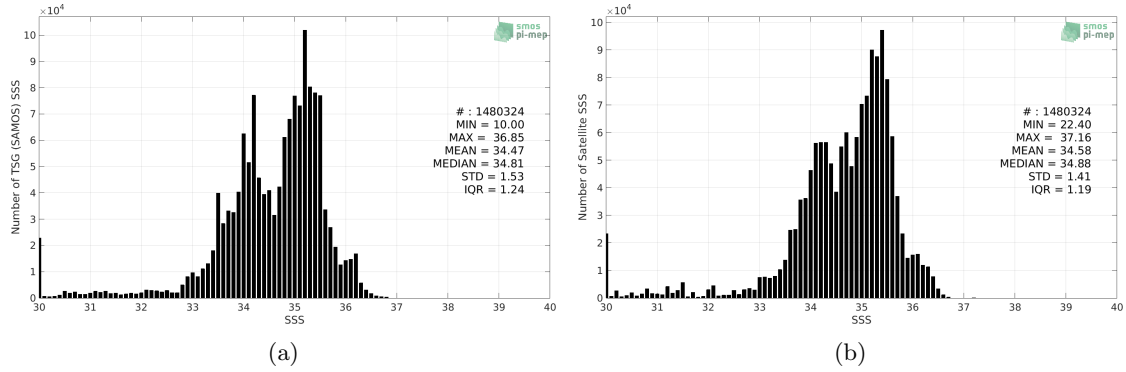
Figure 2: Histograms of SSS from TSG (SAMOS) (a) and SMOS SSS L3 v5 - 18 Days (CATDS-CECOS-LOCEAN) (b) considering all match-up pairs per bins of 0.1 over the Equatorial Ocean 10N-10S Pi-MEP region and for the full satellite product period.
