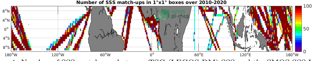
Figure 4: Number of SSS match-ups between TSG (LEGOS-DM) SSS and the SMOS SSS L3 v5 - 18 Days (CATDS-CECOS-LOCEAN) SSS product for the Equatorial Ocean 10N-10S Pi-MEP region over 1^\circ \times 1^\circ boxes and for the full satellite product period.
