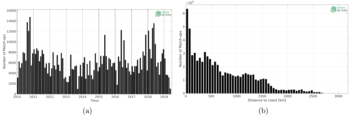
Figure 1: Number of match-ups between TSG (LEGOS-DM) and SMOS SSS L3 v5 - 18 Days (CATDS-CECOS-LOCEAN) SSS as a function of time (a) and as function of the distance to coast (b) over the Equatorial Ocean 10N-10S Pi-MEP region and for the full satellite product period.
