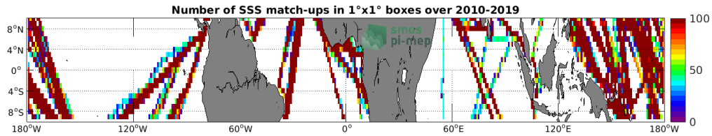
Figure 4: Number of SSS match-ups between TSG (LEGOS-DM) SSS and the SMOS SSS L3 v5 - 18 Days (CATDS-CECOS-LOCEAN) SSS product for the Equatorial Ocean 10N-10S Pi-MEP region over 1^\circ \times 1^\circ boxes and for the full satellite product period.
