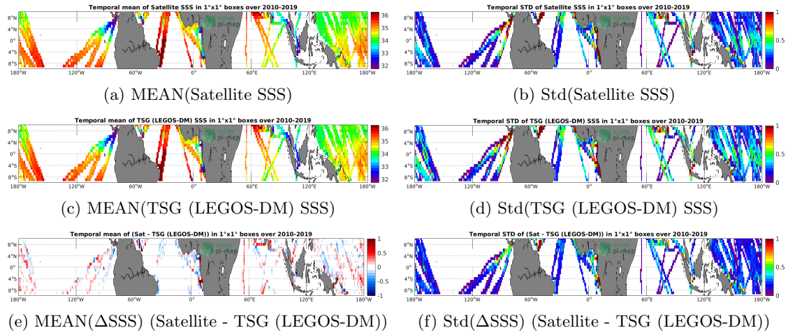
Figure 6: Temporal mean (left) and Std (right) of SSS from SMOS SSS L3 v5 - 18 Days (CATDS-CECOS-LOCEAN) (top), TSG (LEGOS-DM) (middle), and of \Delta SSS (Satellite - TSG (LEGOS-DM)). Only match-up pairs are used to generate these maps.
