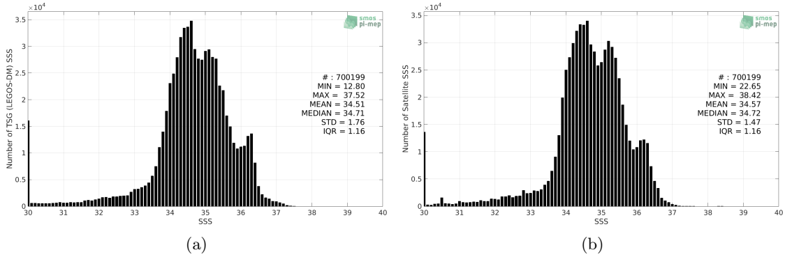
Figure 2: Histograms of SSS from TSG (LEGOS-DM) (a) and SMOS SSS L3 v5 - 18 Days (CATDS-CECOS-LOCEAN) (b) considering all match-up pairs per bins of 0.1 over the Equatorial Ocean 10N-10S Pi-MEP region and for the full satellite product period.
