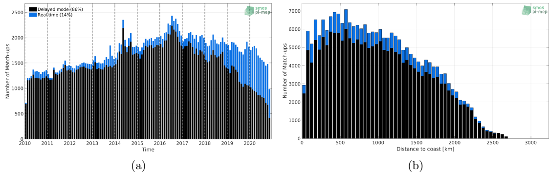
Figure 1: Number of match-ups between Argo and SMOS SSS L3 v5 - 18 Days (CATDS-CECOS-LOCEAN) SSS as a function of time (a) and as function of the distance to coast (b) over the Equatorial Ocean 10N-10S Pi-MEP region and for the full satellite product period.
