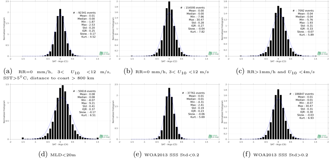
Figure 13: Normalized histogram of \Delta\text{SSS} (SMOS SSS L3 v5 - 18 Days (CATDS-CECOS-LOCEAN) - Argo) for 6 different subdatasets corresponding to: RR=0 mm/h, 3 < U_{10} < 12 m/s, SST>5°C, distance to coast > 800 km (a), RR=0 mm/h, 3 < U_{10} < 12 m/s (b), RR>1mm/h and U_{10} < 4 m/s (c), MLD<20m (d), WOA2013 SSS Std<0.2 (e), WOA2013 SSS Std>0.2 (f).
