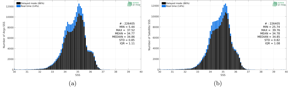
Figure 2: Histograms of SSS from Argo (a) and SMOS SSS L3 v5 - 18 Days (CATDS-CECOS-LOCEAN) (b) considering all match-up pairs per bins of 0.1 over the Equatorial Ocean 10N-10S Pi-MEP region and for the full satellite product period.
