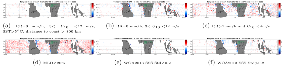
Figure 12: Temporal mean gridded over spatial boxes of size 1^\circ \times 1^\circ of \Delta SSS (SMOS SSS L3 v5 - 18 Days (CATDS-CECOS-LOCEAN) - Argo) for 6 different subdatasets corresponding to: RR=0 mm/h, 3 < U_{10} < 12 m/s, SST > 5^\circ\text{C} , distance to coast > 800 km (a), RR=0 mm/h, 3 < U_{10} < 12 m/s (b), RR > 1 mm/h and U_{10} < 4 m/s (c), MLD < 20 m (d), WOA2013 SSS Std < 0.2 (e), WOA2013 SSS Std > 0.2 (f).
