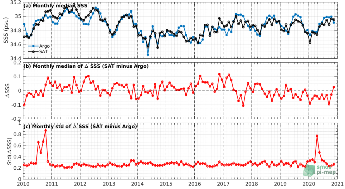
Figure 7: Time series of the monthly median SSS (top), median of \Delta\text{SSS} (Satellite - Argo) and Std of \Delta\text{SSS} (Satellite - Argo) over the Equatorial Ocean 10N-10S Pi-MEP region considering all match-ups collected by the Pi-MEP.
