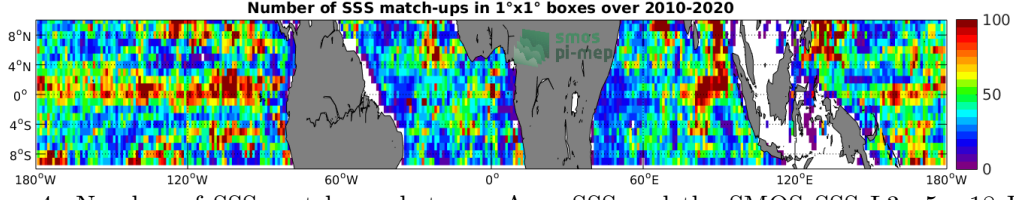
Figure 4: Number of SSS match-ups between Argo SSS and the SMOS SSS L3 v5 - 18 Days (CATDS-CECOS-LOCEAN) SSS product for the Equatorial Ocean 10N-10S Pi-MEP region over 1^\circ \times 1^\circ boxes and for the full satellite product period.
