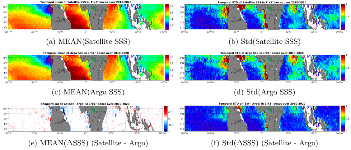
Figure 6: Temporal mean (left) and Std (right) of SSS from SMOS SSS L3 v5 - 18 Days (CATDS-CECOS-LOCEAN) (top), Argo (middle), and of \Delta SSS (Satellite - Argo). Only match-up pairs are used to generate these maps.
