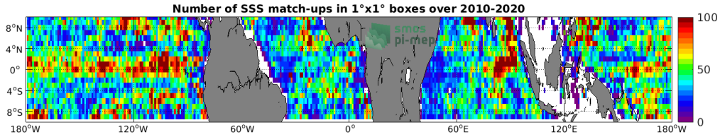
Figure 4: Number of SSS match-ups between Argo SSS and the SMOS SSS L3 v5 - 18 Days (CATDS-CECOS-LOCEAN) SSS product for the Equatorial Ocean 10N-10S Pi-MEP region over 1^\circ \times 1^\circ boxes and for the full satellite product period.
