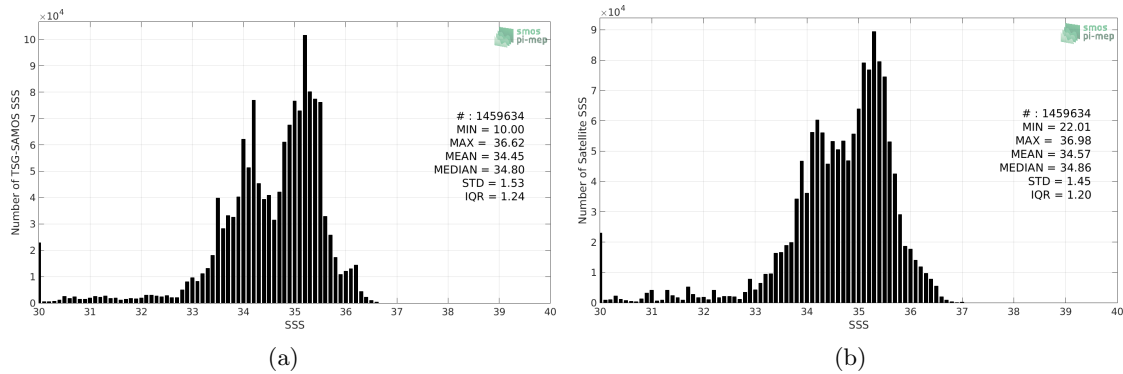
Figure 2: Histograms of SSS from TSG-SAMOS (a) and SMOS-L3-CATDS-CECOS-LOCEAN-V4-9DAYS-25KM (b) considering all match-up pairs per bins of 0.1 over the Equatorial Ocean 10N-10S Pi-MEP region and for the full satellite product period.
