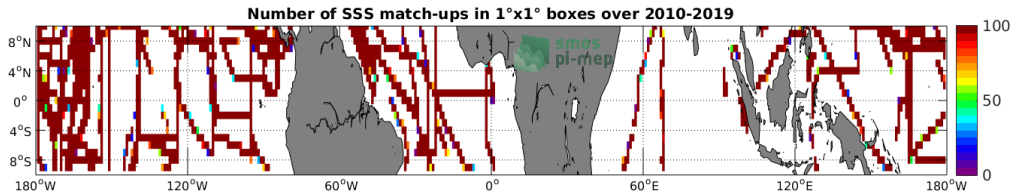
Figure 4: Number of SSS match-ups between TSG-SAMOS SSS and the SMOS-L3-CATDS-CECOS-LOCEAN-V4-9DAYS-25KM SSS product for the Equatorial Ocean 10N-10S Pi-MEP region over 1°x1° boxes and for the full satellite product period.
