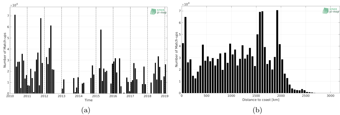
Figure 1: Number of match-ups between TSG-SAMOS and SMOS-L3-CATDS-CECOS-LOCEAN-V4-9DAYS-25KM SSS as a function of time (a) and as function of the distance to coast (b) over the Equatorial Ocean 10N-10S Pi-MEP region and for the full satellite product period.
