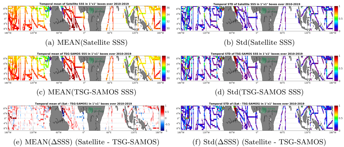
Figure 6: Temporal mean (left) and Std (right) of SSS from SMOS-L3-CATDS-CECOS-LOCEAN-V4-9DAYS-25KM (top), TSG-SAMOS (middle), and of \Delta SSS (Satellite - TSG-SAMOS). Only match-up pairs are used to generate these maps.
