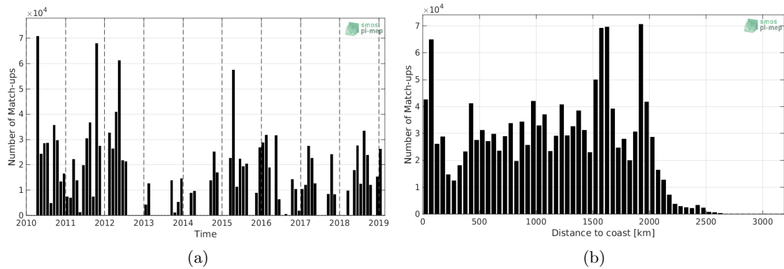
Figure 1: Number of match-ups between TSG-SAMOS and SMOS-L3-CATDS-CECOS-LOCEAN-V4-9DAYS-25KM SSS as a function of time (a) and as function of the distance to coast (b) over the Equatorial Ocean 10N-10S Pi-MEP region and for the full satellite product period.
