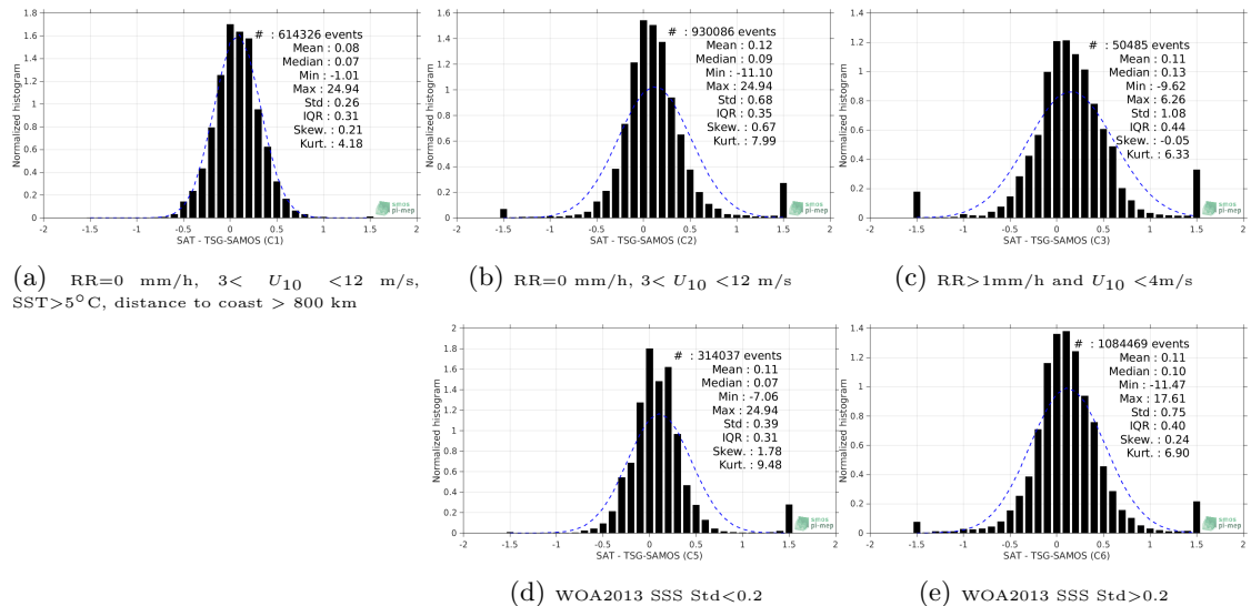
Figure 13: Normalized histogram of \Delta SSS (SMOS-L3-CATDS-CECOS-LOCEAN-V4-9DAYS-25KM - TSG-SAMOS) for 5 different subdatasets corresponding to: RR=0 mm/h, 3 < U_{10} < 12 m/s, SST >5^\circ C, distance to coast > 800 km (a), RR=0 mm/h, 3 < U_{10} < 12 m/s (b), RR >1 mm/h and U_{10} < 4 m/s (c), WOA2013 SSS Std <0.2 (d), WOA2013 SSS Std >0.2 (e).
