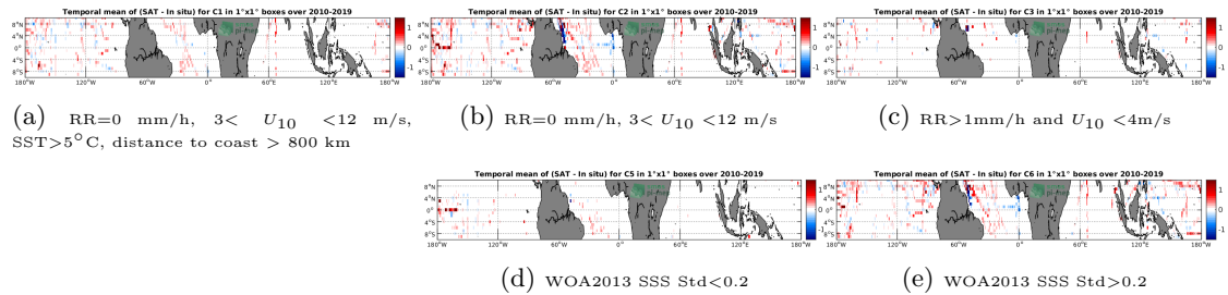
Figure 12: Temporal mean gridded over spatial boxes of size 1^\circ \times 1^\circ of \Delta SSS (SMOS-L3-CATDS-CECOS-LOCEAN-V4-9DAYS-25KM - TSG-SAMOS) for 5 different subdatasets corresponding to: RR=0 mm/h, 3 < U_{10} < 12 m/s, SST >5^\circ C, distance to coast > 800 km (a), RR=0 mm/h, 3 < U_{10} < 12 m/s (b), RR >1 mm/h and U_{10} < 4 m/s (c), WOA2013 SSS Std <0.2 (d), WOA2013 SSS Std >0.2 (e).
