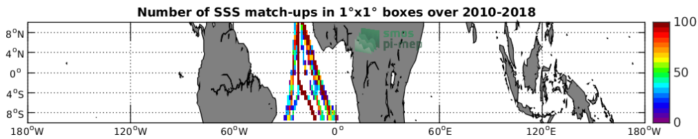
Figure 4: Number of SSS match-ups between TSG-POLARSTERN SSS and the SMOS-L3-CATDS-CECOS-LOCEAN-V4-9DAYS-25KM SSS product for the Equatorial Ocean 10N-10S Pi-MEP region over 1°x1° boxes and for the full satellite product period.
